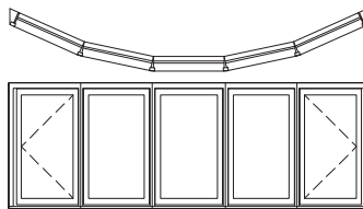
Five Wide Casement Bow
