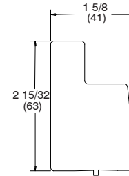
W1075 – Hinged Screen Mull Casing
