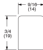
W1080 – Mull Filler (Spline)
