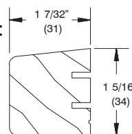
W6064 – Head Jamb Space Block (In-sash Transom)
