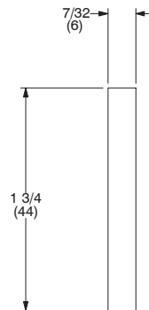
W6248 – Mull Filler*
