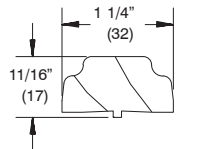
W7554 – Astragal Cover and Transom Mull Cover – Wood
