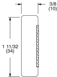
W7531 – Jamb Filler – 6 9/16" jambs (with adhesive tape)*
