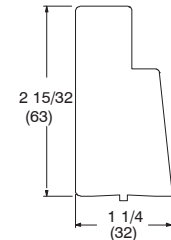
W1452 – Sliding Screen Mull Casing (4 9/16" Jamb) – Wood
