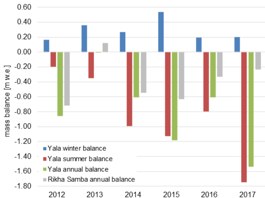
465 Figure 4: Winter, summer and annual mass balance of Yala Glacier and annual balance of Rikha Samba Glacier, calculated based on the respective gradients. In the mass-balance years 2011/12 and 2014/15, the sum of winter and summer balances differ significantly from the annual balances, likely due to a lack of data in higher elevations.
