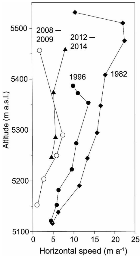
Figure 12: Altitudinal distribution of the surface flow speeds of Yala Glacier, surveyed in 1982 by Ageta et al. (1984), 1996 by Fujita et al. (1998), 2008 to 2009 by Sugiyama et al. (2013) and from 2012 to 2014 in this study (adapted from Fujita et al. 1998).
