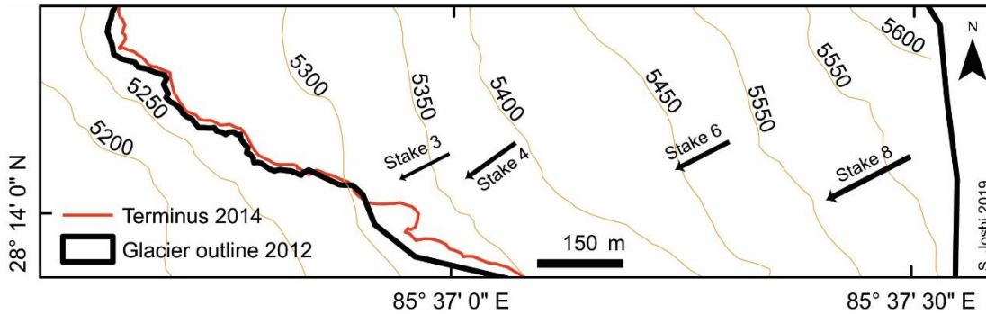
Figure 11: Glacier flow from 8 May 2012 to 5 May 2014 at the stakes 3, 4, 6 and 8, with annual rates between 4.6 and 7.8 \text{ m a}^{-1} . The black arrows show the flow direction and the lengths indicate the annual speed of glacier surface flow, which is depicted 10 times longer than the real flow (Figure adapted from Sugiyama et al., 2013).
