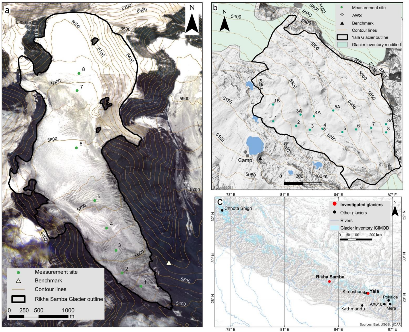
125 Figure 1: The study sites Rikha Samba and Yala glaciers showing the measurement sites and their location in the Himalayas. At all measurements sites stakes were installed. Snow pits were dug at the top stakes and at selected lower stakes provided snow was present. (a) For Rikha Samba Glacier RapidEye orthoimages from April 2010 were used for the background image and glacier outlines. The contour lines are derived from the SRTM-3 DEM. (b) For Yala Glacier GeoEye-1 orthoimages from January 2012 were used for the background image and in combination with dGNSS data for the glacier outlines. The contour lines are derived from the DEM2012 generated from the GeoEye-1 stereo images. (c) The overview map shows the location of the two investigated 130 glaciers and other glaciers mentioned in the discussion section. The glacier inventory is from ICIMOD (Bajracharya et al., 2014).
