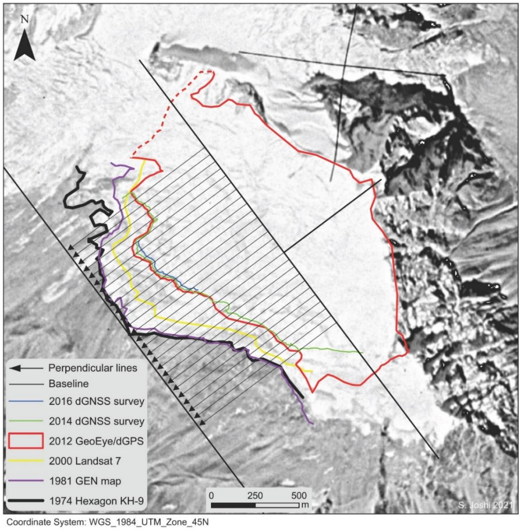
565 Figure 9: Frontal variations of Yala Glacier from 1974 to 2016. The general flow direction is indicated by a straight black line starting at the highest point of the glacier (north-east corner). An arbitrary baseline marks the maximum extent of 1974. Twenty-six parallel arrows in flow direction at 50 m intervals were used to calculate average frontal variations but to exclude outliers only the 9 lines crossing the terminus from 2016 were used for the analysis. The background image is the Hexagon KH-9 from 1974.
