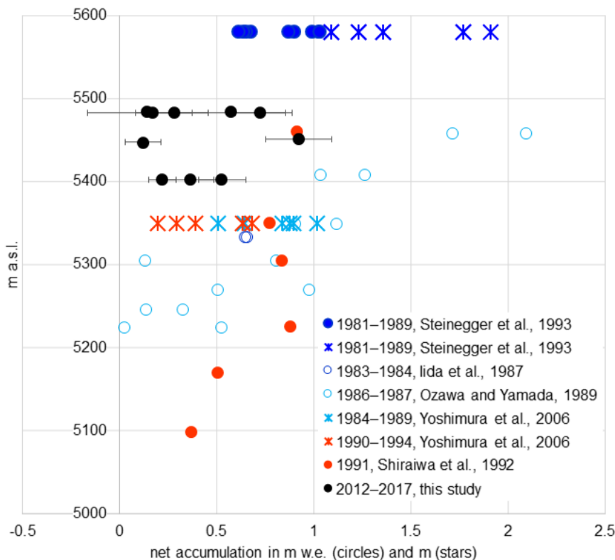
810 Figure 14: Positive point mass balances in the accumulation area from mass-balance years in the 1980s (blue), 1990s (red) and from this study (black). The data was compiled from annual snow pit measurements, multiannual snow profiles, ice cores and crevasses, using dirt, algae or ice layers to distinguish annual layers. Most measurements were converted into water equivalents (circles), and
