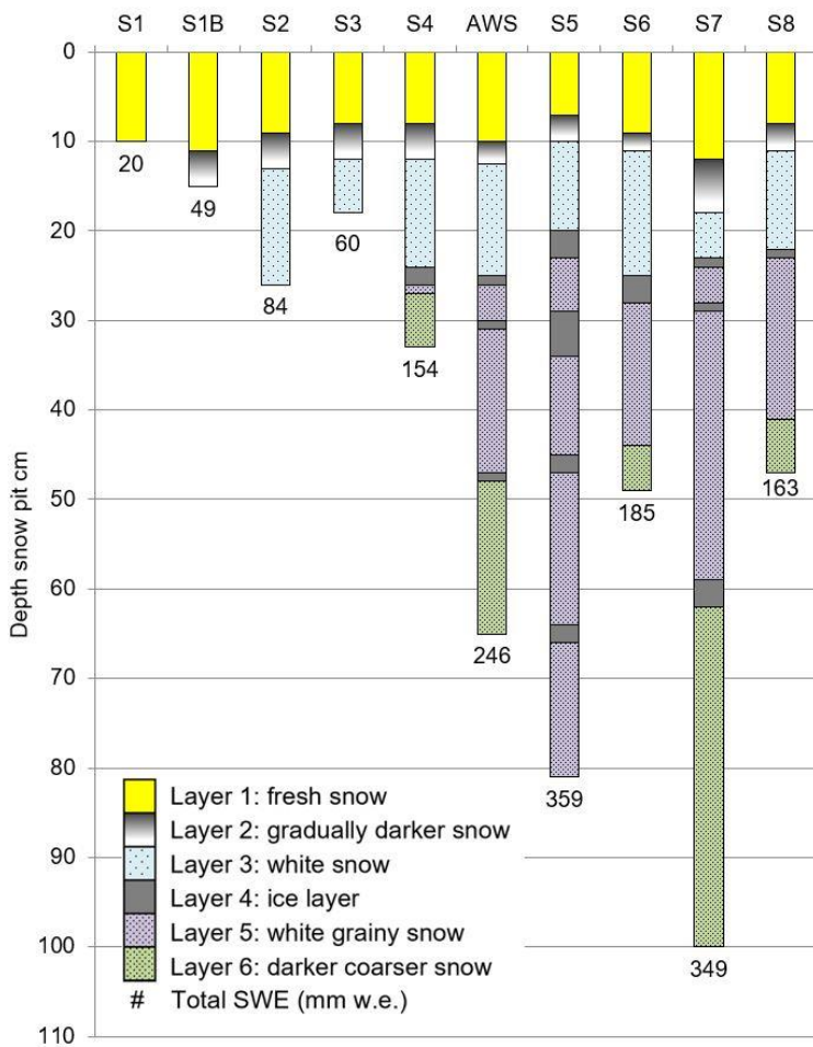
515 Figure 6: Snow profiles measured at the stakes on Yala Glacier on 23, 24 and 25 April 2017. At the site AWS, a temporary weather station was set up near stake S4. Distinct snow layers can be identified at all measurement sites. At the stakes S5, S6, S7, and S8 sawdust from 19 and 20 November 2016 was found at the bottom of the snow pit, and glacier ice at all lower sites.
