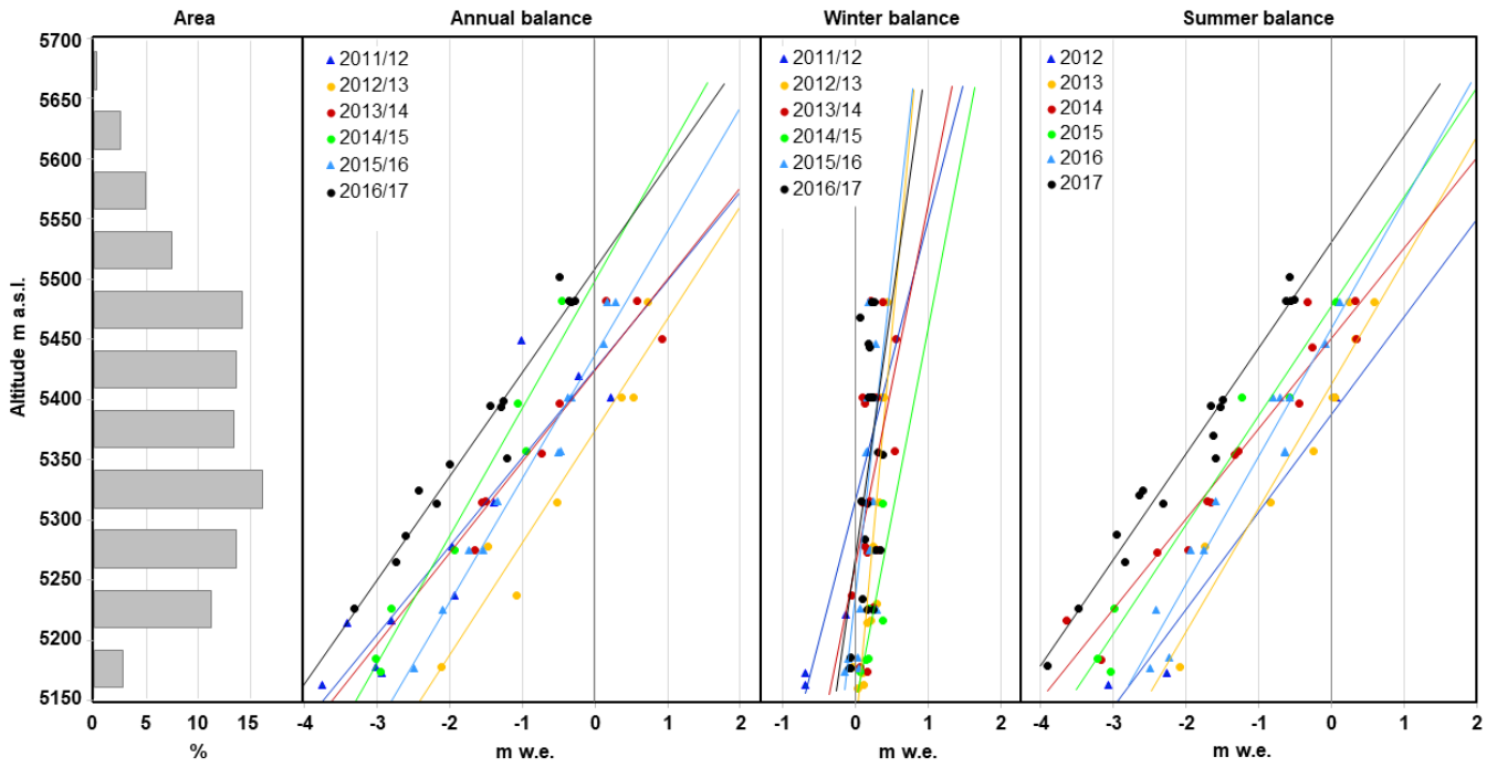
450 Figure 2: Mass balances and gradients for the annual, winter and summer mass balance for Yala Glacier from 2011–2017, and the glacier hypsography (far left).
