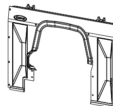
COWL ASS'Y. P/N: 8SV-GC179505-R3
