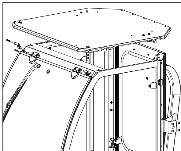
Fig. 12.1 (Roof Installation)
