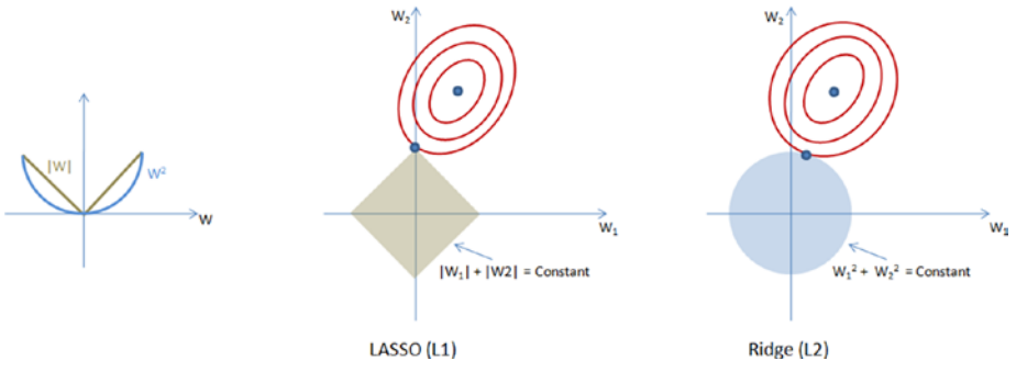
Figure 3-9. Regularizations
