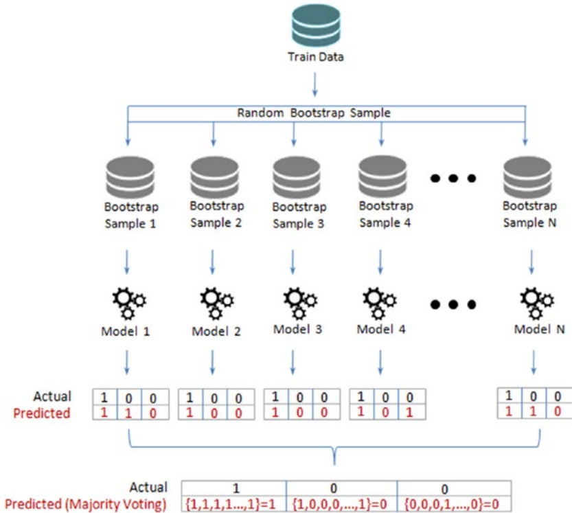
Figure 4-6. Bagging
