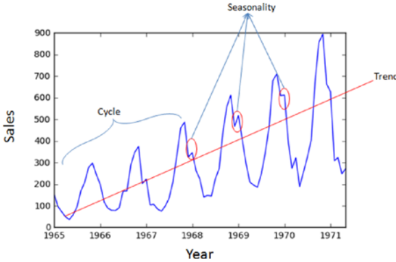
Figure 3-17. Time series components
