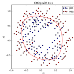
Right-fitting
