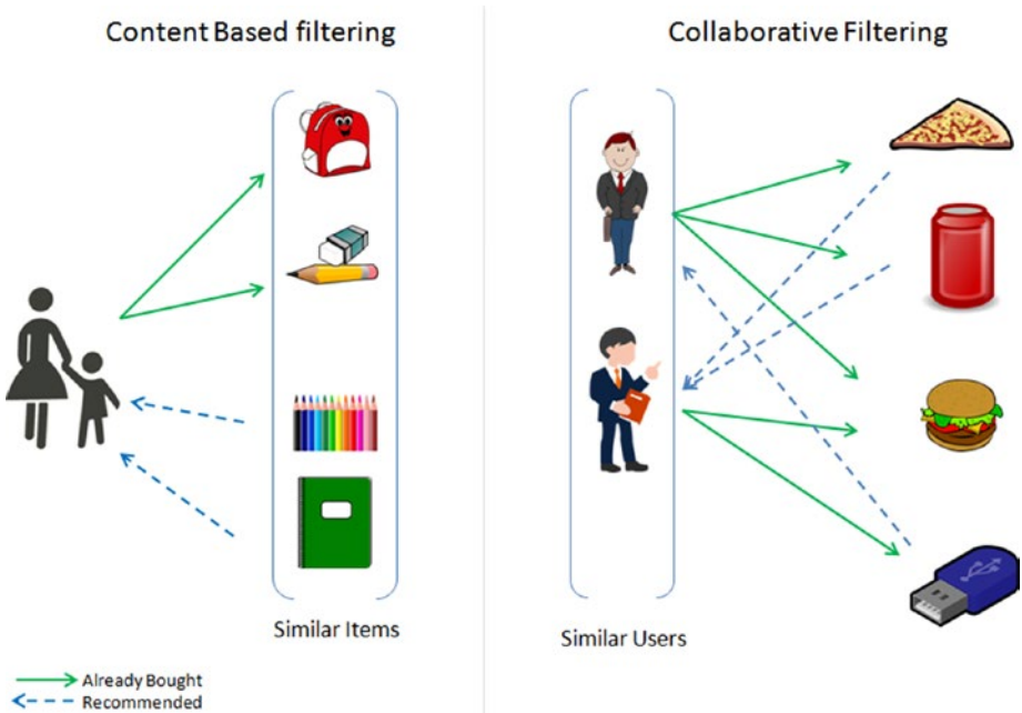
Figure 5-10. Recommender systems
