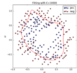
Over-fitting
