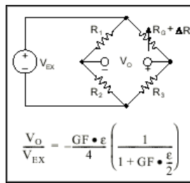
Figure 4. Quarter-Bridge Circuit
