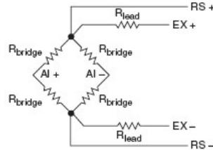
Figure 9b. Remote Sensor Error Compensation
