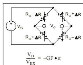
Figure 7. Full-Bridge Circuit
