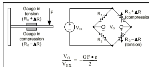
Figure 6. Half-Bridge Circuit
