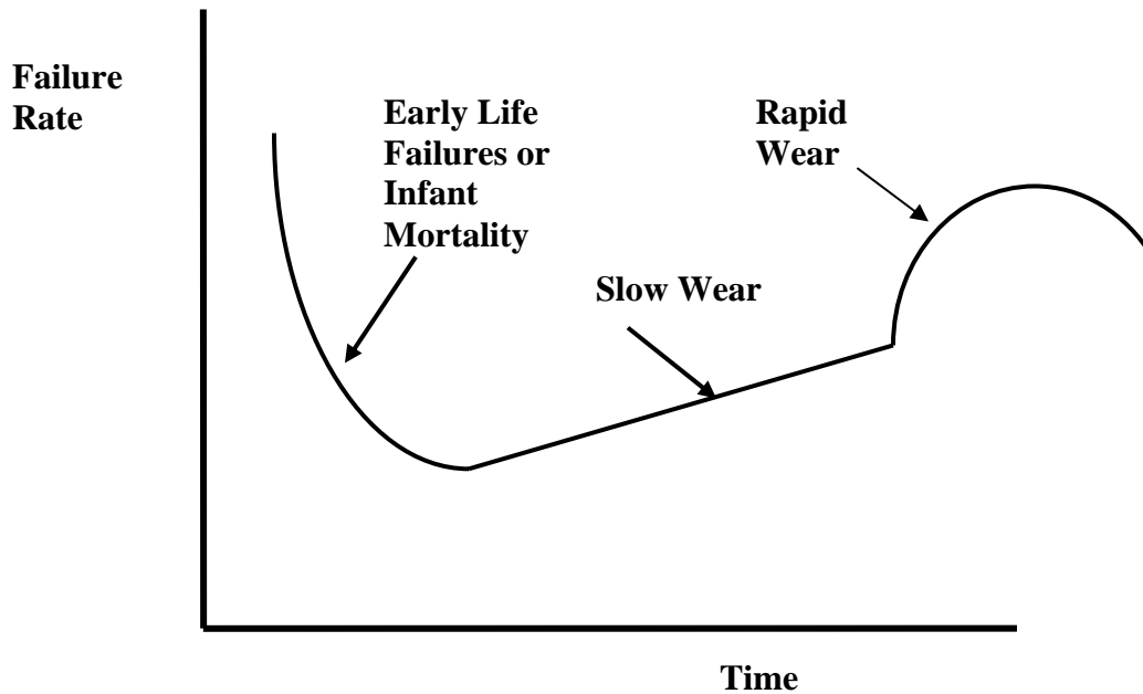
Figure 5.9 – Slow Wear of a Mechanical Bathtub Curve
