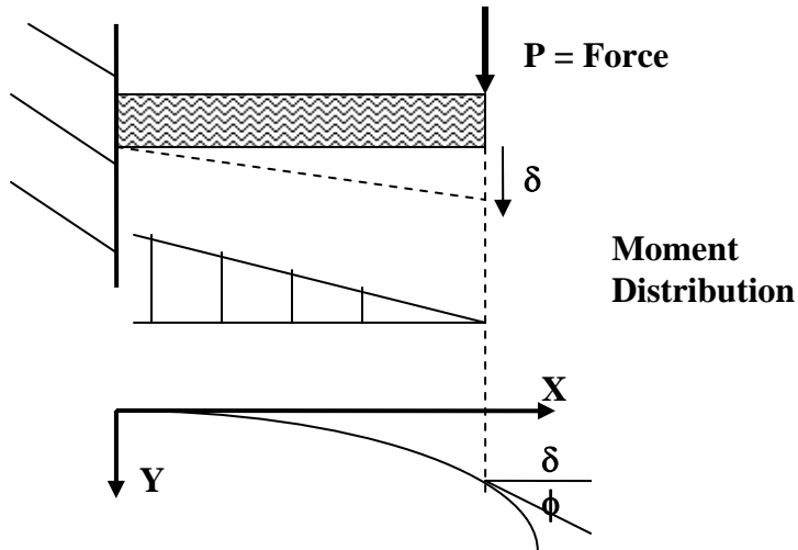
Figure 1.10 – The Free End of a Beam under and End Load
