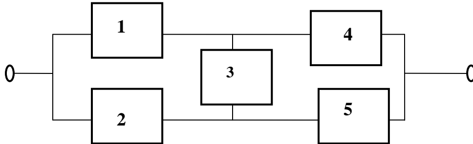
Figure 5.7 – A Complex System
