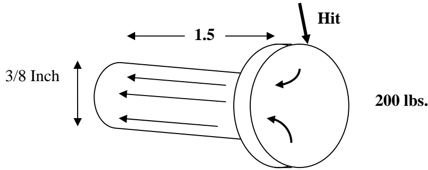
Figure 4.5 - Actuator Example
