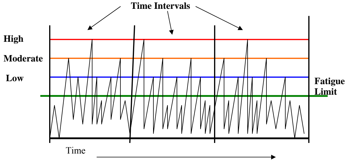
Figure 3.2 – The Summary of Stresses Observed over Three Time Periods
