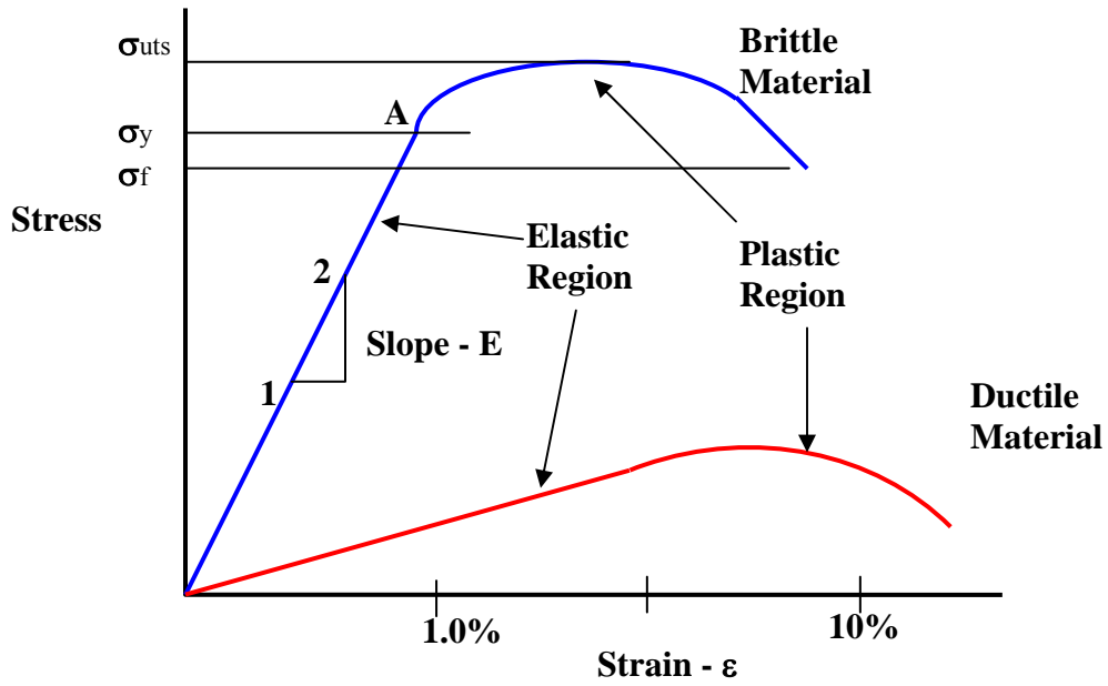
Figure 1.1a - The Stress-Strain Diagram
