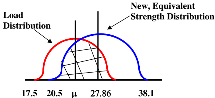
Figure 3.10 – An Equivalent Normal Distribution for Strength
