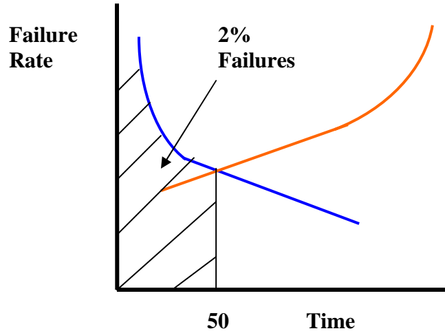
Figure 4.2 – The Spliced Early Portion of the Bathtub Curve
