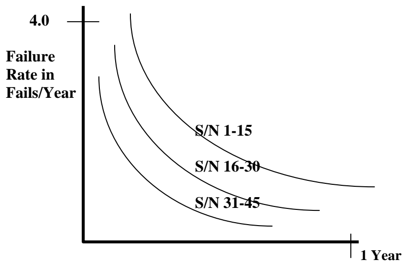
Figure A7 – Performance of Successive Production Lots by Serial Number of System A
