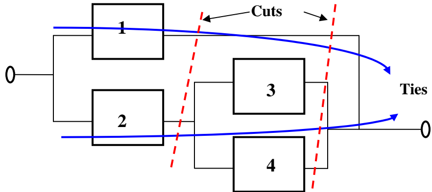
Figure 5.6 – Cut Sets and Ties Sets
