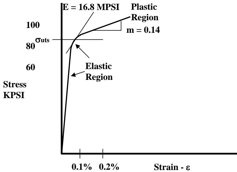
Figure 1.1b - An Alternate Stress-Strain Diagram for Annealed, A40 Titanium
