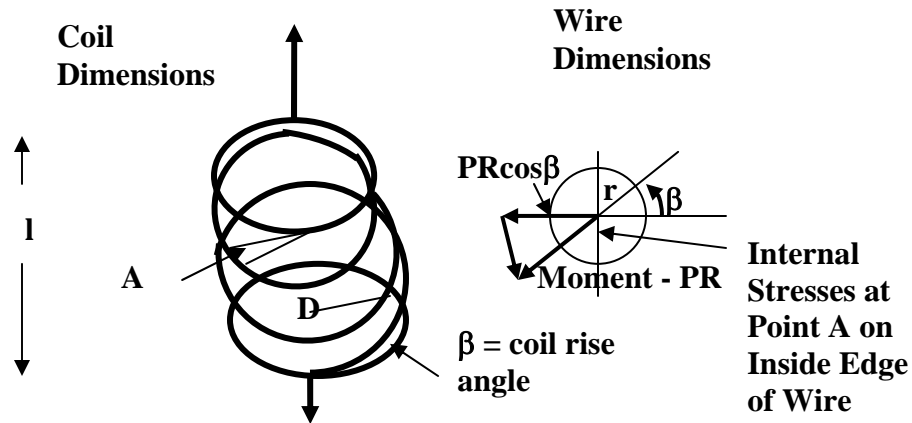
Figure 1.8 – The Helical Spring
