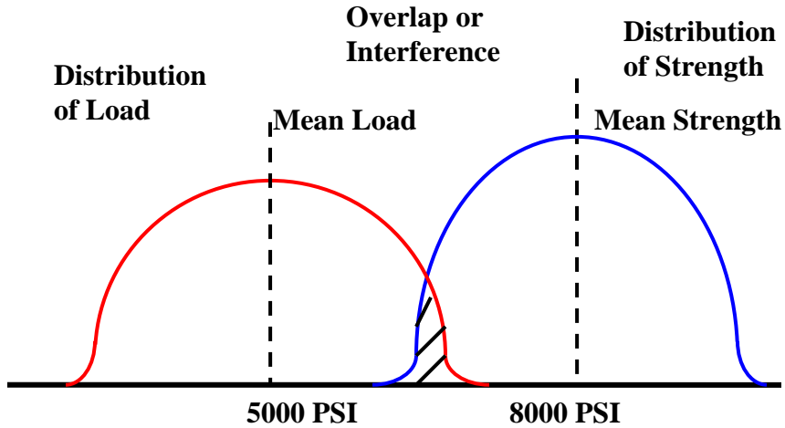
Figure 1.12 – The Stress–Load Model
