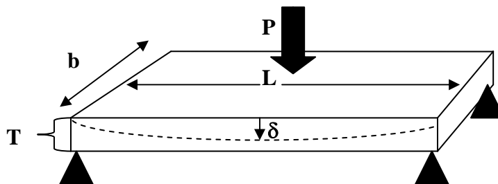
Figure 5.1 – The Deflection of a Wide Beam under Load
