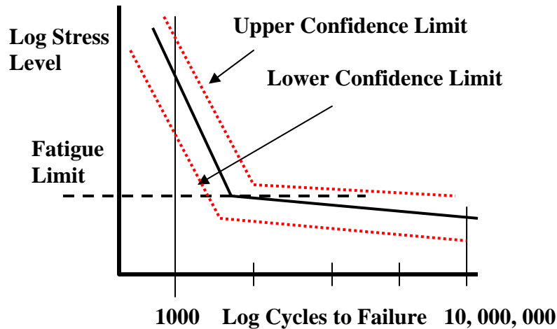
Figure 3.7 – Confidence Limits on the S-N Curve
