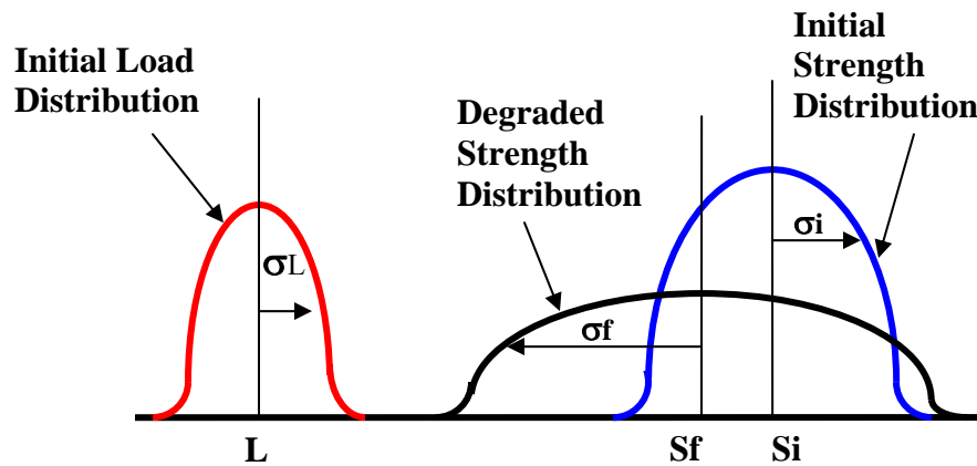
Figure 3.1 - The Stress-Load Degradation Model
