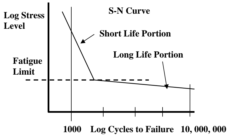
Figure 3.4 – The S-N Curve
