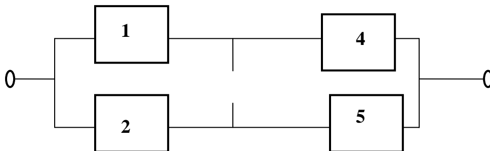
Figure 5.8B – When Component Three Fails
