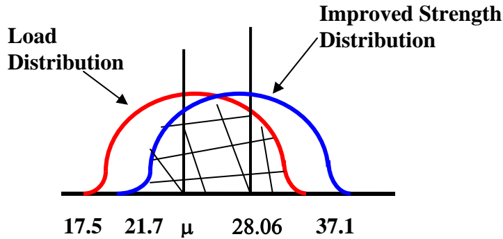
Figure 3.11 – An Improved Normal Distribution for Strength
