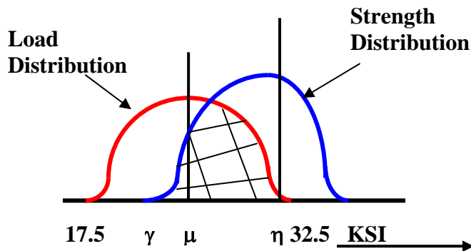
Figure 3.9 – Interference of the Normal and Weibull Distribution
