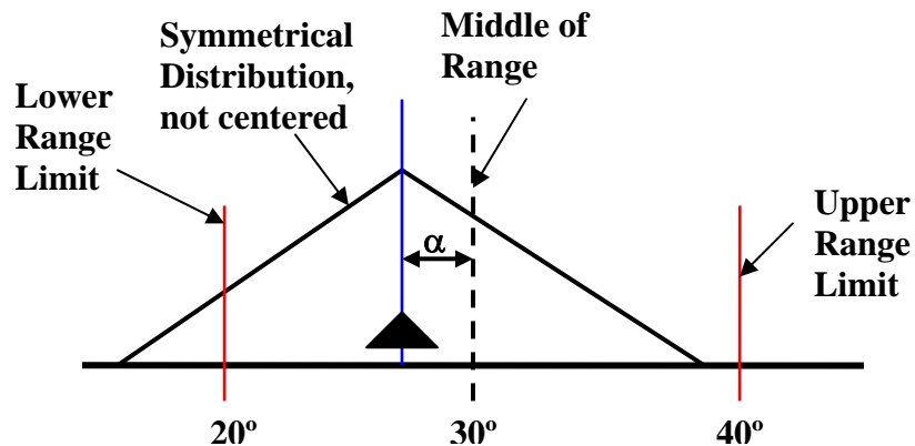
Figure 5.3 – Gauss' Inequality Model
