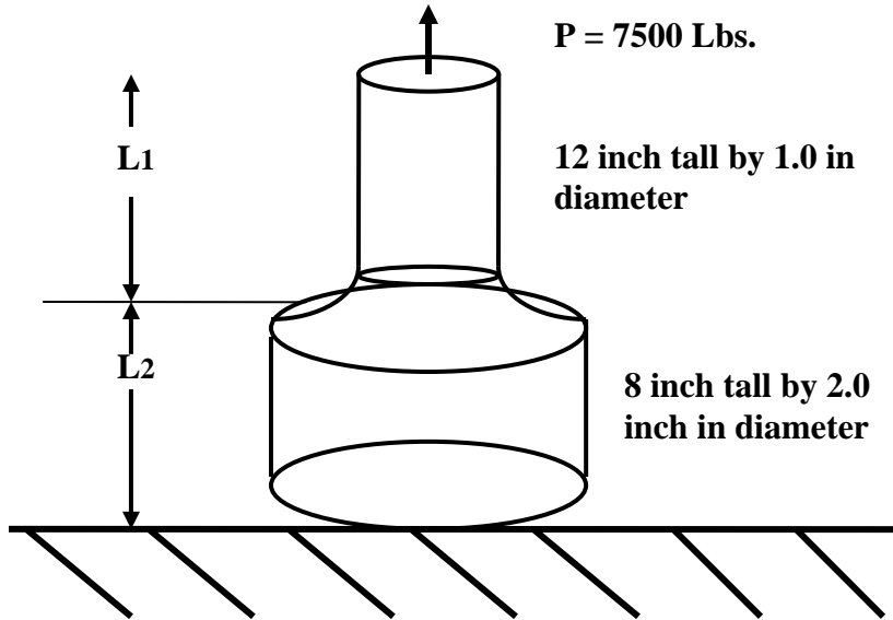
Figure1.5 – A Tapered Shaft with a Load
