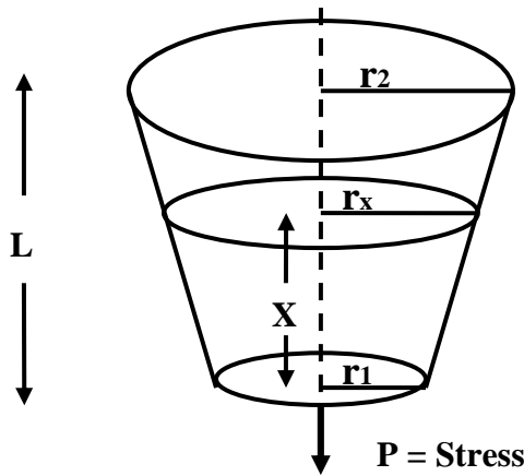
Figure 1.2 - A Truncated Cone
