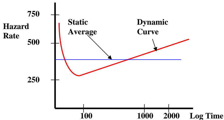
Figure 4.3 – A Dynamic Hazard Rate Curve
