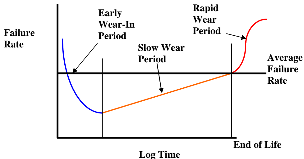
Figure 4.1 – The Mechanical Bathtub Curve
