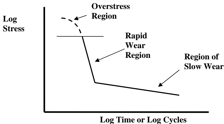
Figure 5.10 – The Dual Stress-Life Relationship
