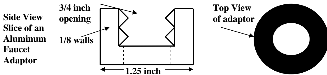
Figure 4.4 – An Aluminum Faucet Adaptor
