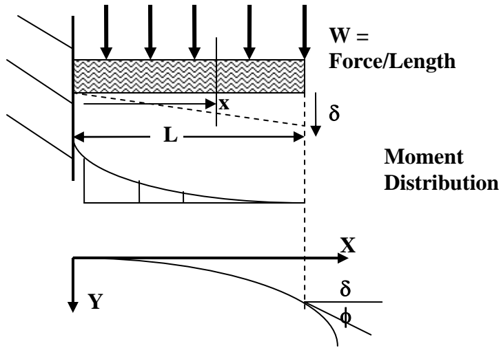
Figure 1.11- A Beam under a Uniform Load
