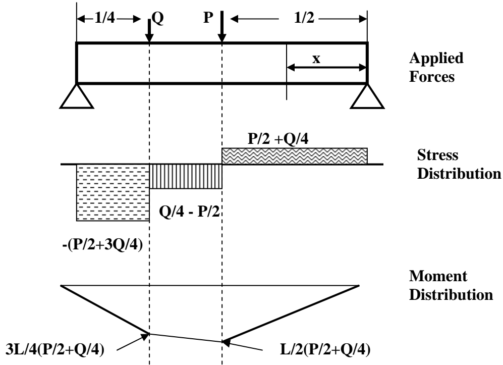
Figure 1.9 – The Stress Distribution in a Beam
