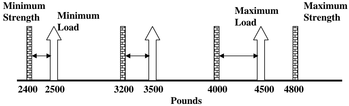
Figure 5.12 – The Distribution of Strength and Load
