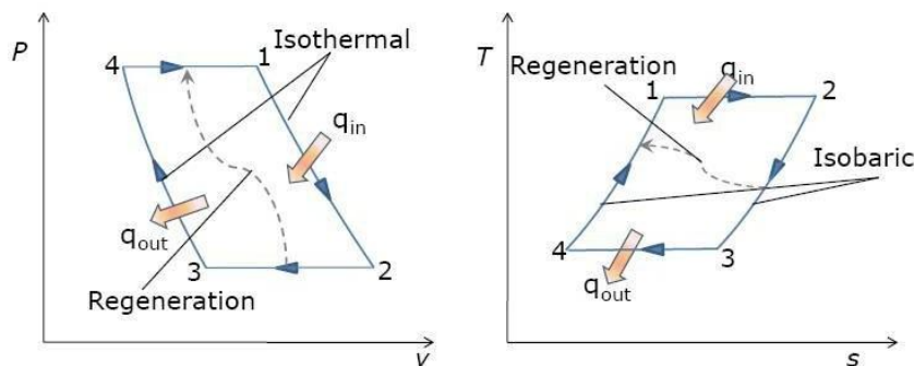
Ericsson cycle on P-v and T-s diagrams
