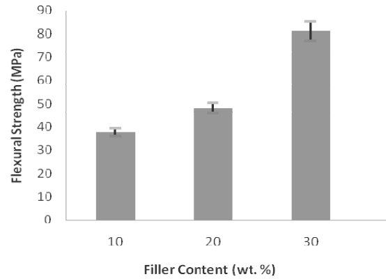
Fig. 5. Flexural strength of the composite samples containing various amounts of nm-size \text{Al}_2\text{O}_3 filler particles
