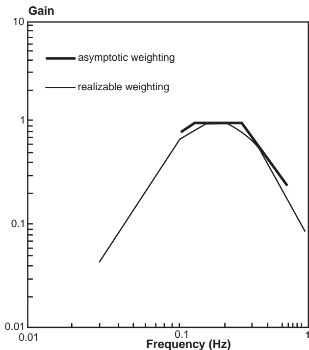
Fig. 35-9. Bode plot of the filter characteristic required to provide the frequency weighting ( W_f ) used to calculate the motion sickness dose value ( MSDV_z ) in the equation MSDV_z = a \cdot W_f \cdot t^{1/2} (Equation 1 in the chapter). The graph shows a straight-line “asymptotic approximation” used to define the weighting function, as is required in the specification of measuring instruments, and the “realizable weighting” that can be achieved by conventional electronic filters. The weighting function has the characteristic of a band-pass filter with the greatest sensitivity in the octave 0.125–0.25 Hz with rapid attenuation in sensitivity at higher and lower frequencies. Reproduced with permission from Griffin MJ. Physical characteristics of stimuli provoking motion sickness. In: Motion Sickness: Significance in Aerospace Operations and Prophylaxis . Neuilly-sur-Seine, France: Advisory Group for Aerospace Research and Development, North Atlantic Treaty Organization. 1991; Paper 3:3-11. AGARD Lecture Series 175.
