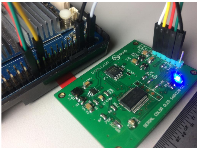
Figure 2 – SPI wiring up close
