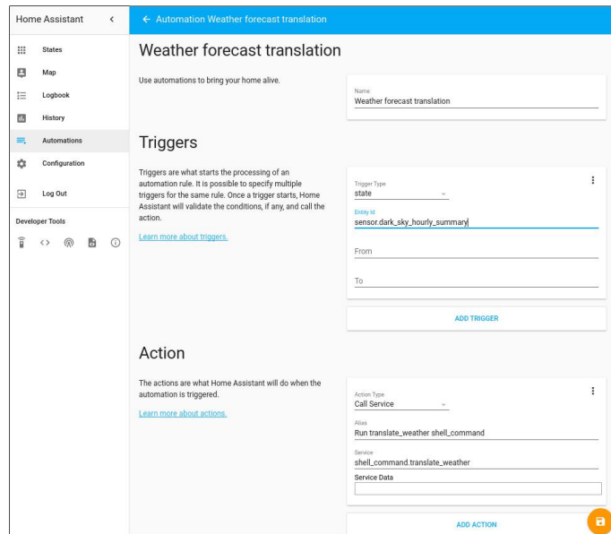
Figure 5 - Create a new automation
