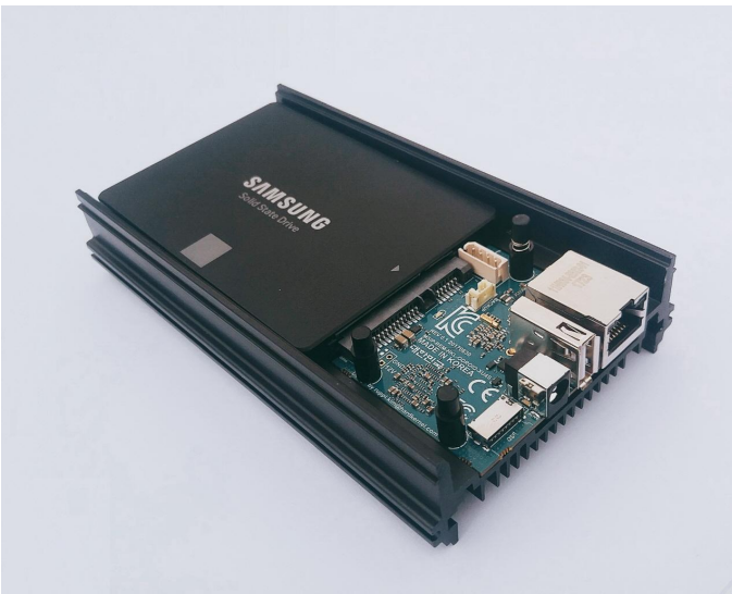
The ODROID-HC1 is an elegant, affordable solution to home cloud computing
