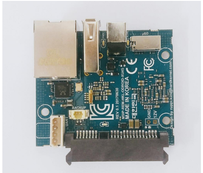
The SoC and PMIC are glued with epoxy resin to increase their reliability
