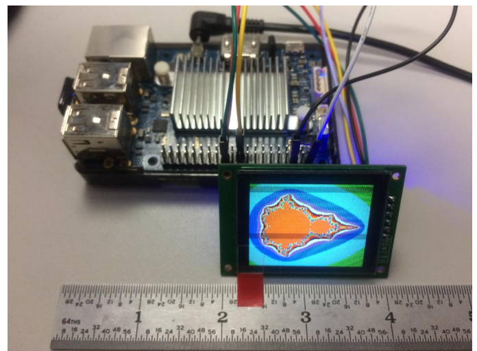
Figure 1 - Dougherty's mandel.c test in SPI 3-wire mode. Scan lines in photos are not visible to the human eye.
