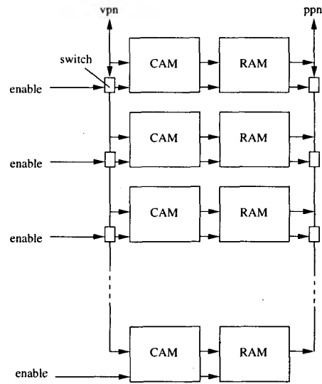
Figure 4. The organization of the configurable TLB
