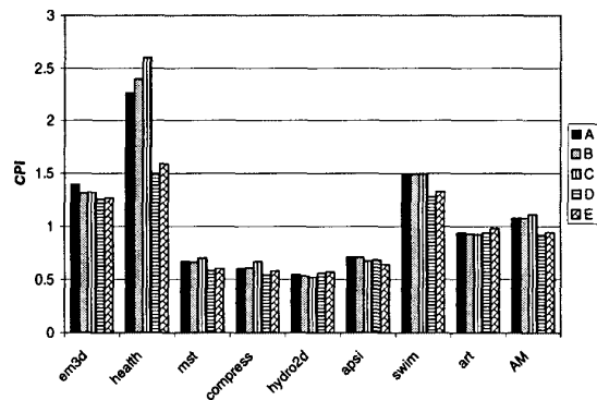
Figure 6. CPI for conventional (A, B, and C), interval-based (D), and subroutine-based (E) configurable schemes
