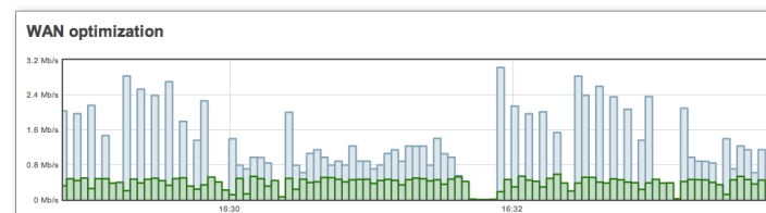
WAN Optimization
