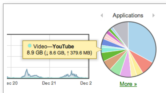
Application Control
