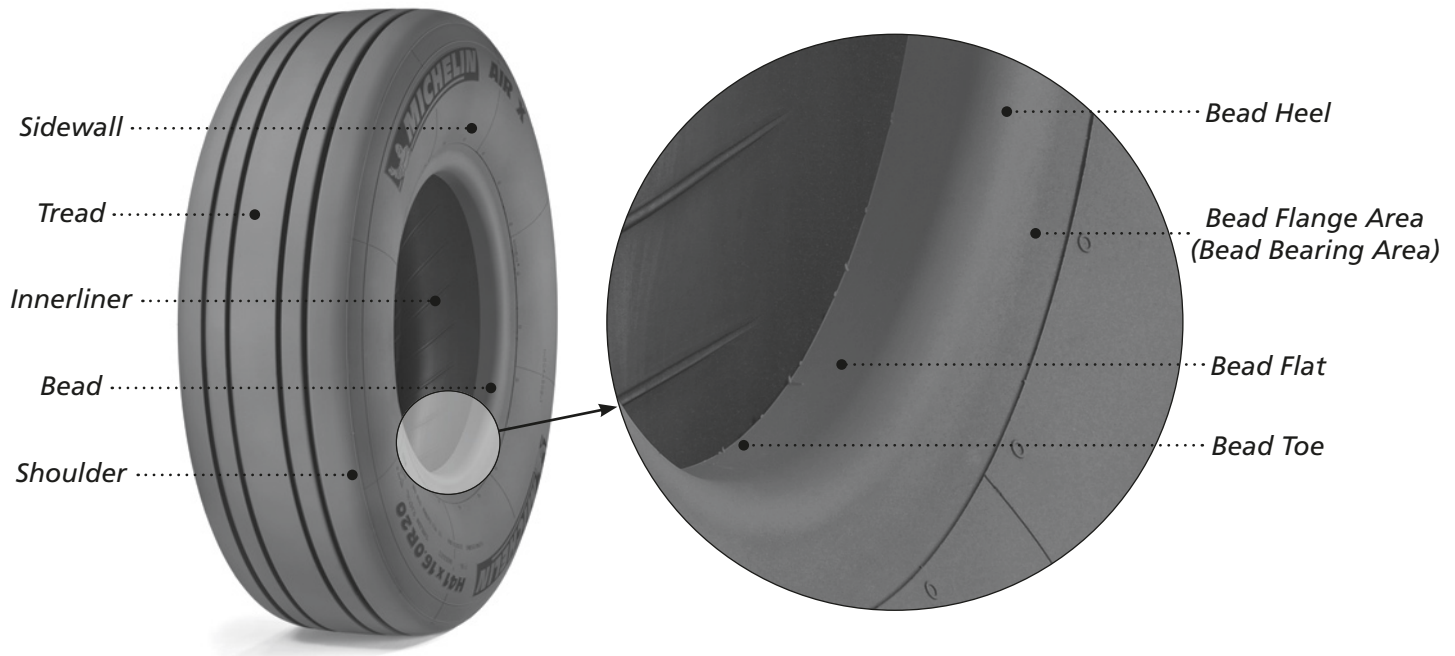
Figure 101. Tire Zones and Tire Bead Zones
