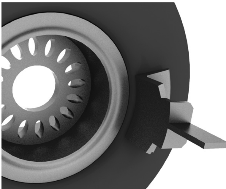
Figure 605. Pincher-Type Bead Breaker
