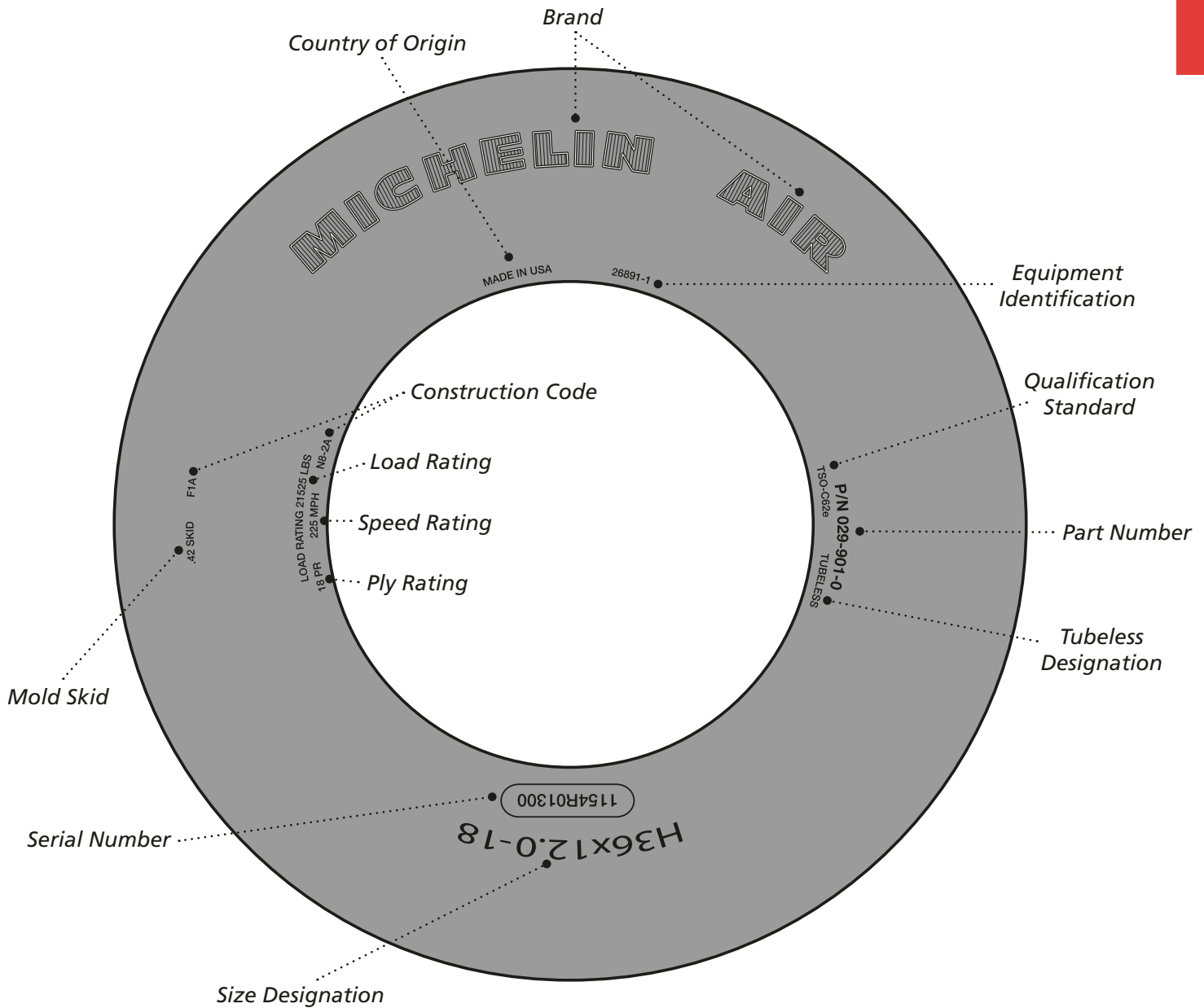
Figure 202. Typical Aircraft Tire Markings – Civil Bias
