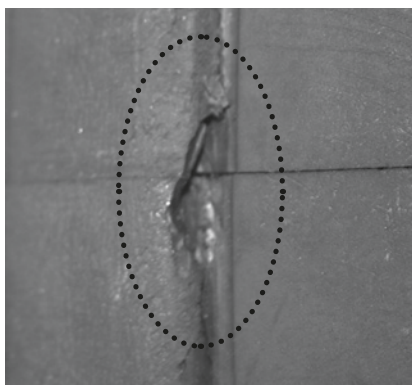
Figure 521. Rib Undercutting
