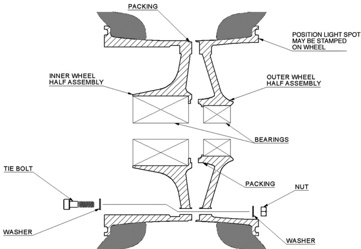
Figure 406. Aircraft Tire/Wheel Assembly
