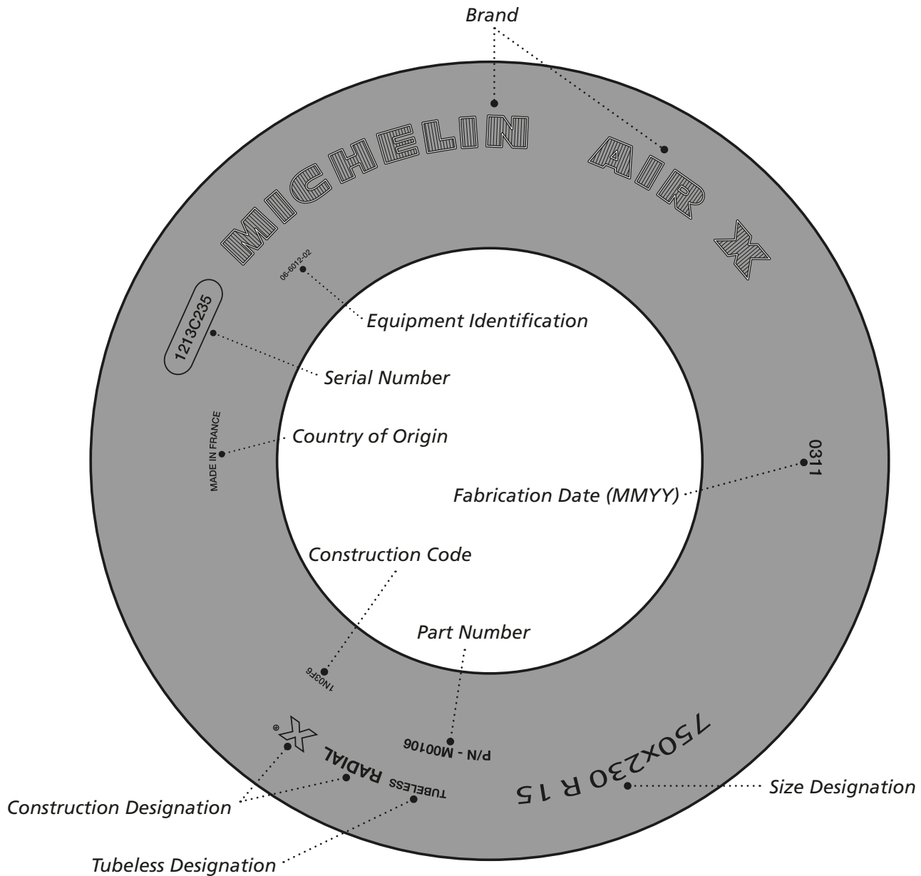
Figure 204. Typical Aircraft Tire Markings – Military Radial, Non-US
