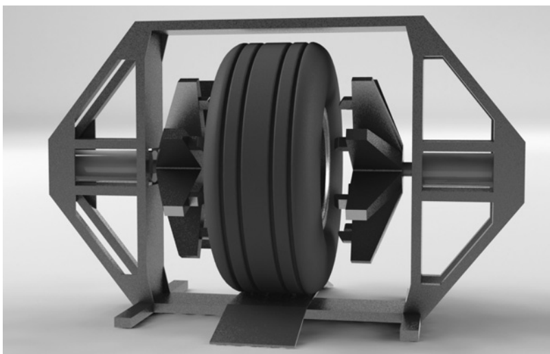
Figure 604. Finger-Type Bead Breaker
