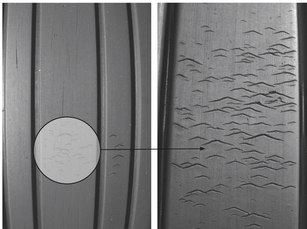
Figure 514. Chevron Cutting
