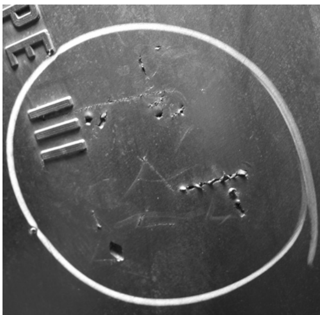
Figure 302. Damage From Contact With Sharp Object - Serviceable
