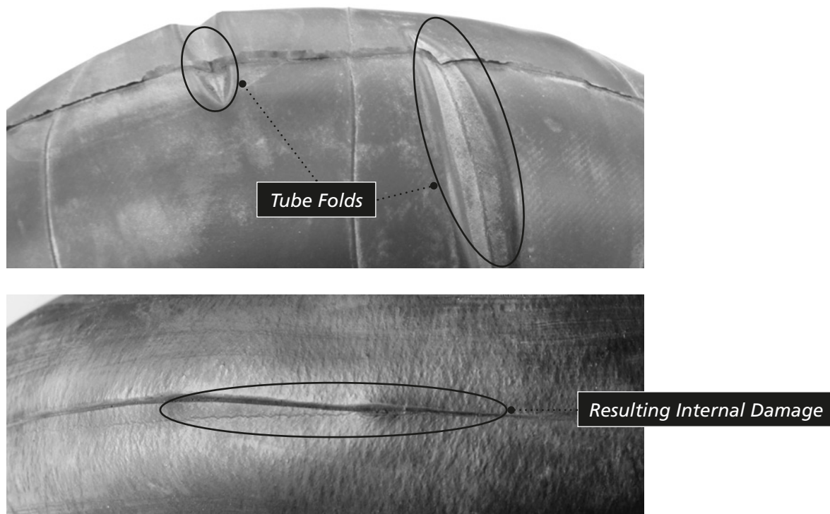
Figure 407. Example of Tube Folds
