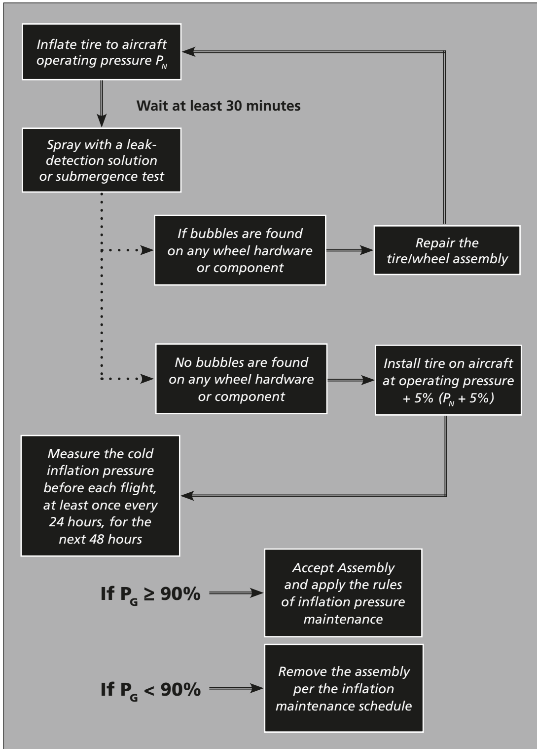
Figure 411. Emergency Pressure-Retention Procedure
