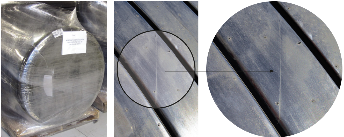
Figure 304. Damage From a Knife Cut
