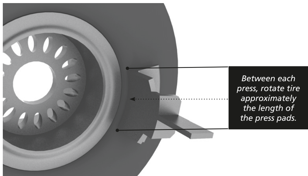
Figure 609. Rotation Between Pressings
