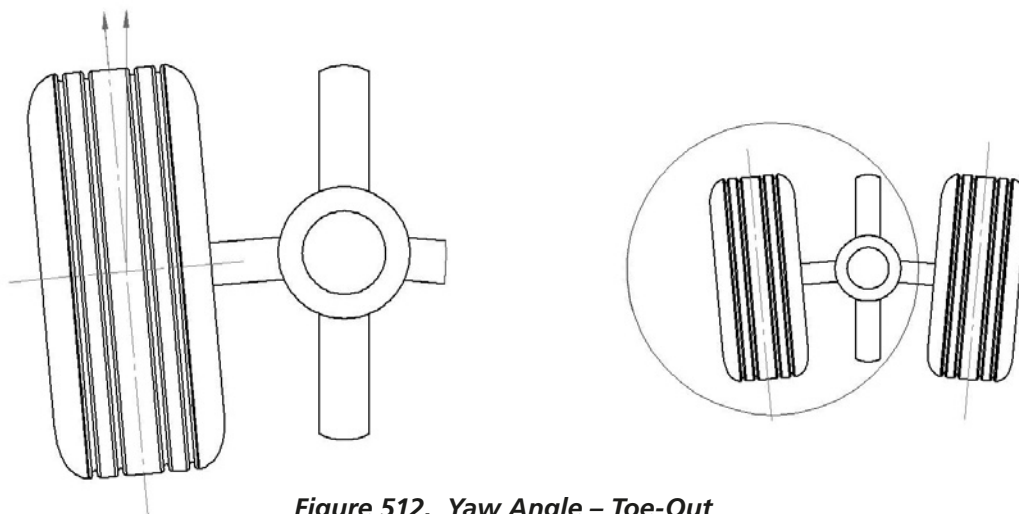
Figure 512. Yaw Angle – Toe-Out
