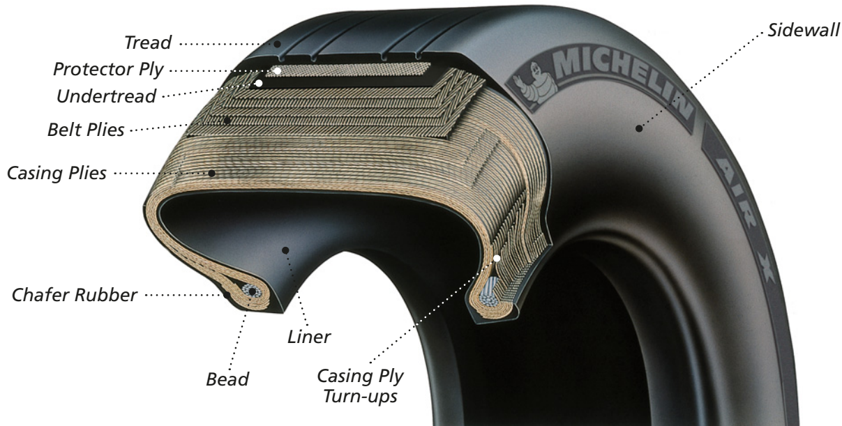
Figure 102. Radial Aircraft Tire
