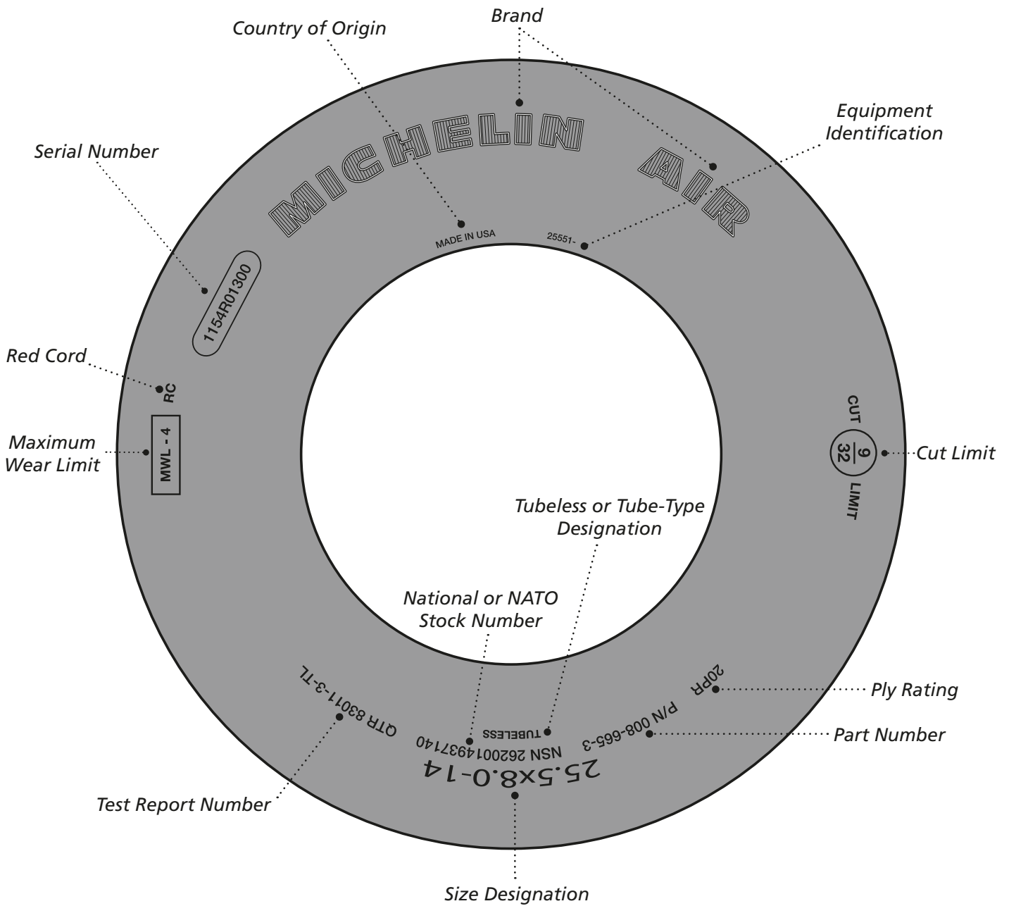
Figure 205. Typical Aircraft Tire Markings – Military Bias
