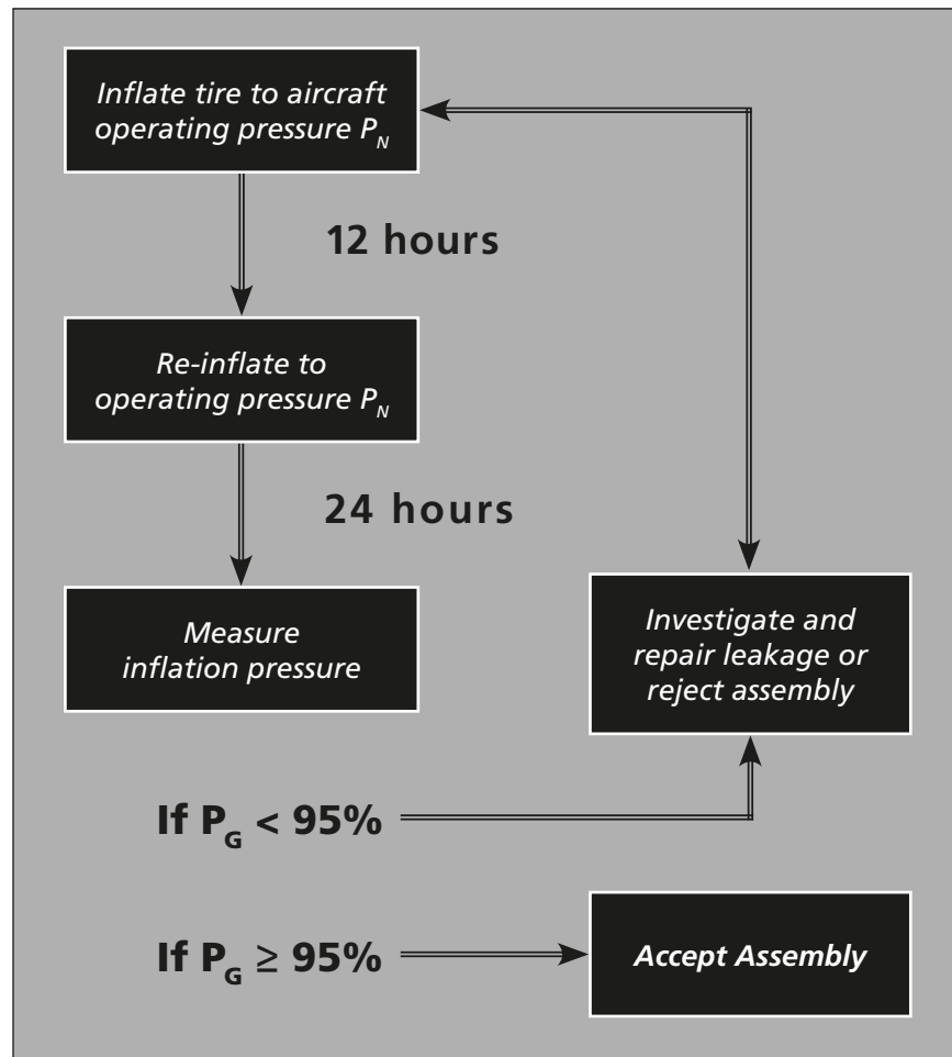
Figure 409. Industry Standard Pressure-Retention Procedure
