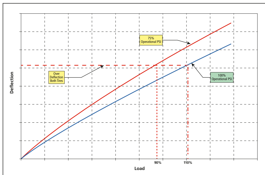
Figure 502. Effect of Unequal Pressure on Tire Loads
