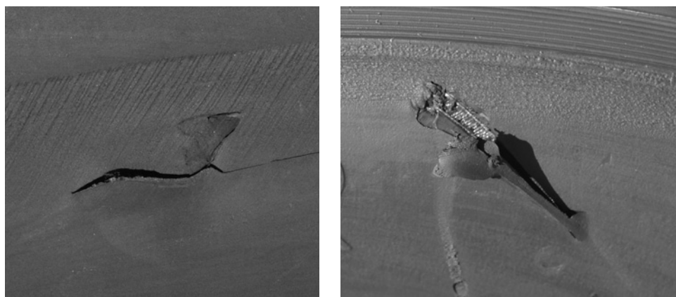
Figure 525. Sidewall FOD – Remove From Service (exposed cords)
