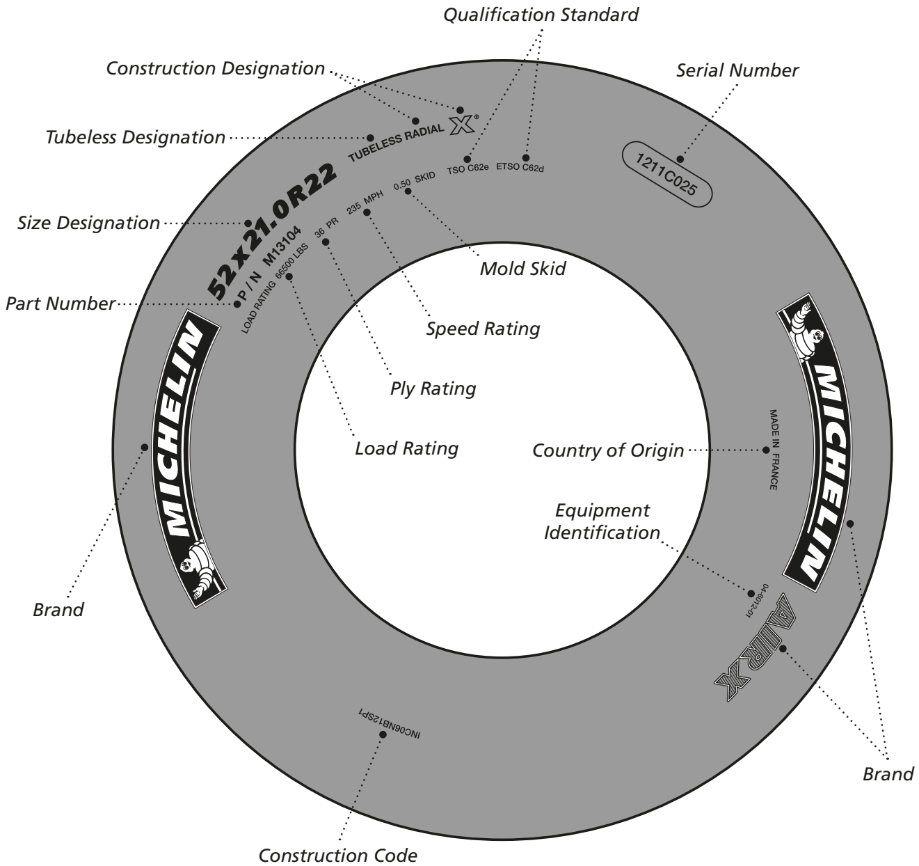
Figure 201. Typical Aircraft Tire Markings – Civil Radial
