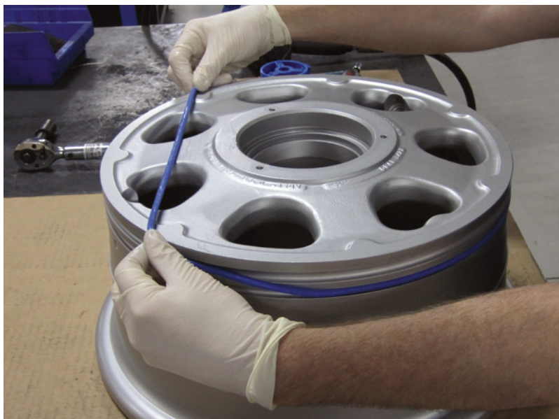
Figure 404. Installation of O-Ring on Inner Wheel Half
