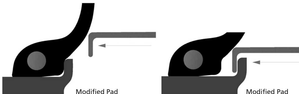
Figure 612. Modified Press Pad for Pincher-Type Bead Breakers
