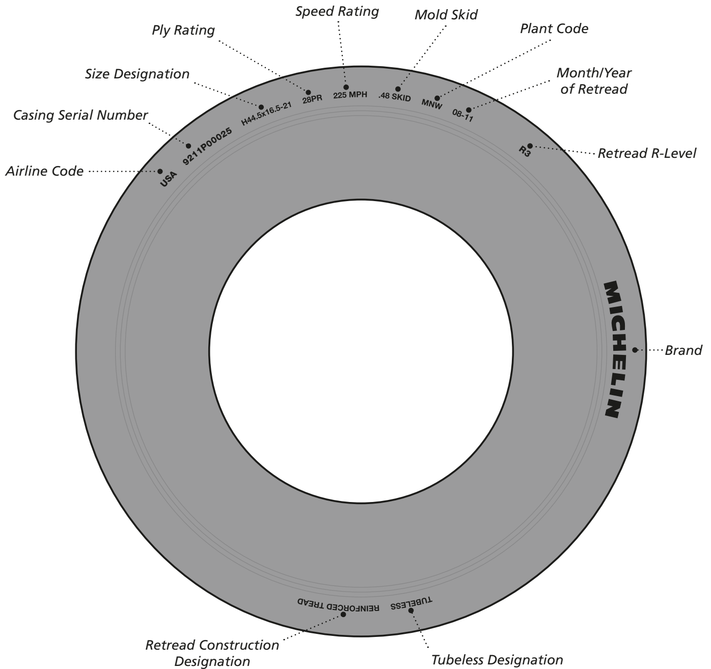
Figure 206. Typical Retread Aircraft Tire Markings
