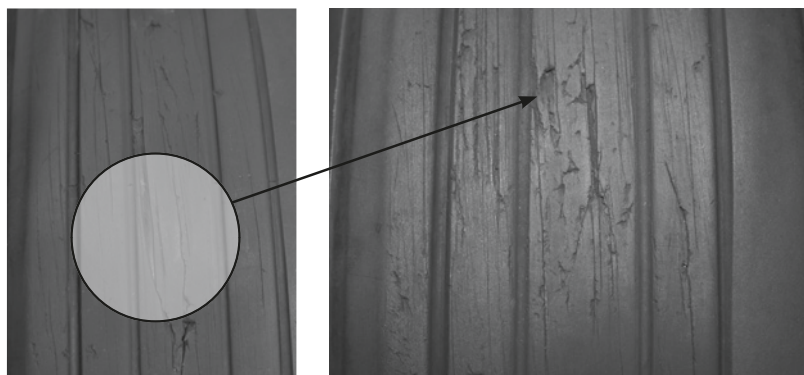
Figure 519. Tread Chunking
