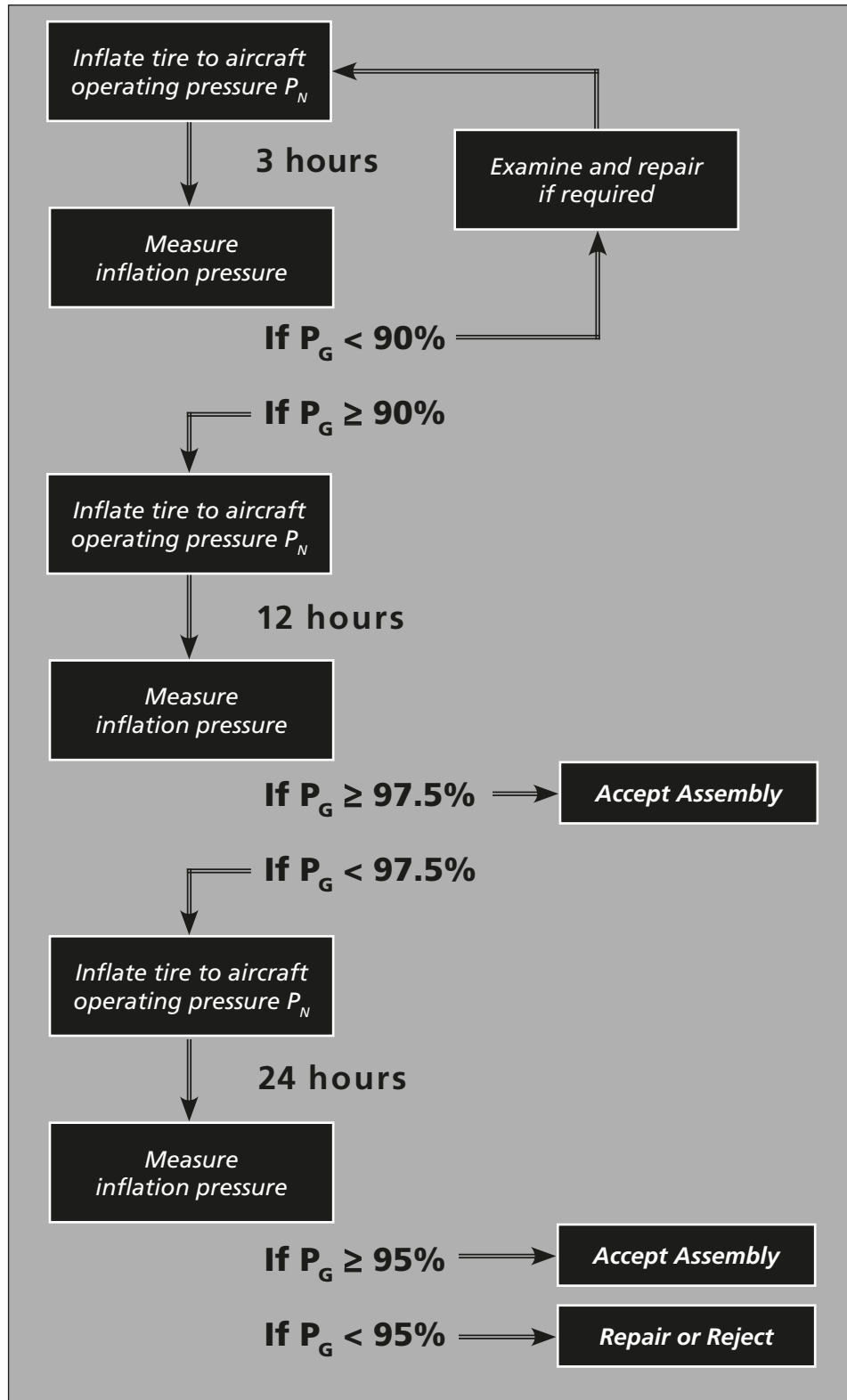
Figure 410. Alternate Pressure-Retention Procedure
