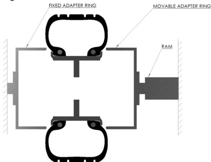
Figure 603. Ring-Type Bead Breaker
