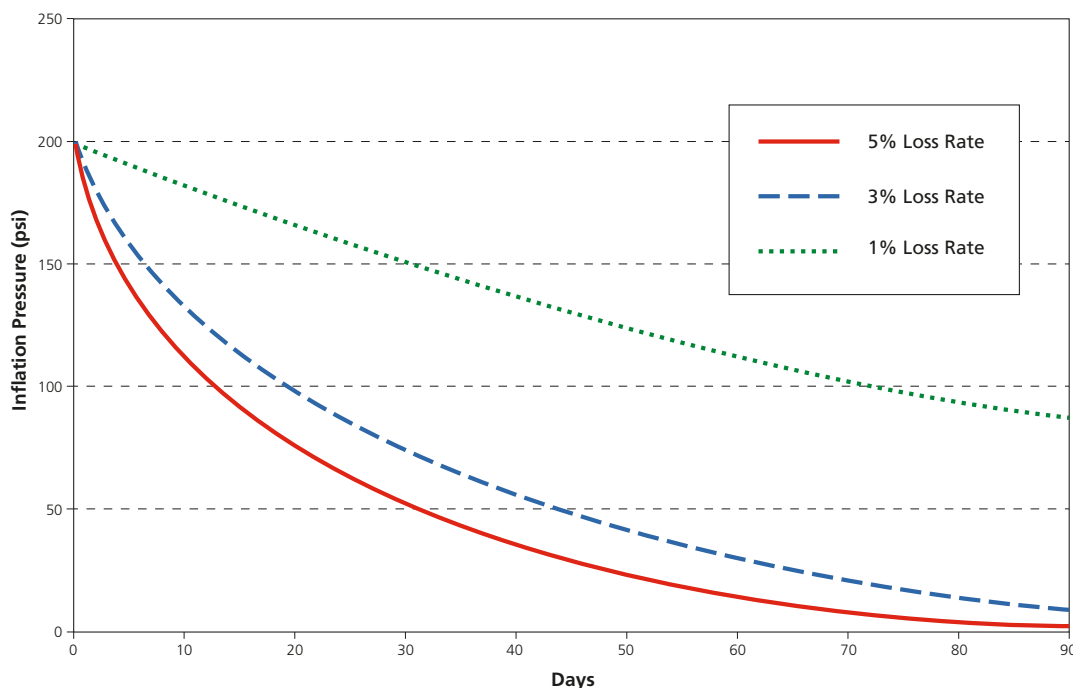
Figure 413. Tire Pressure Loss Over Time
