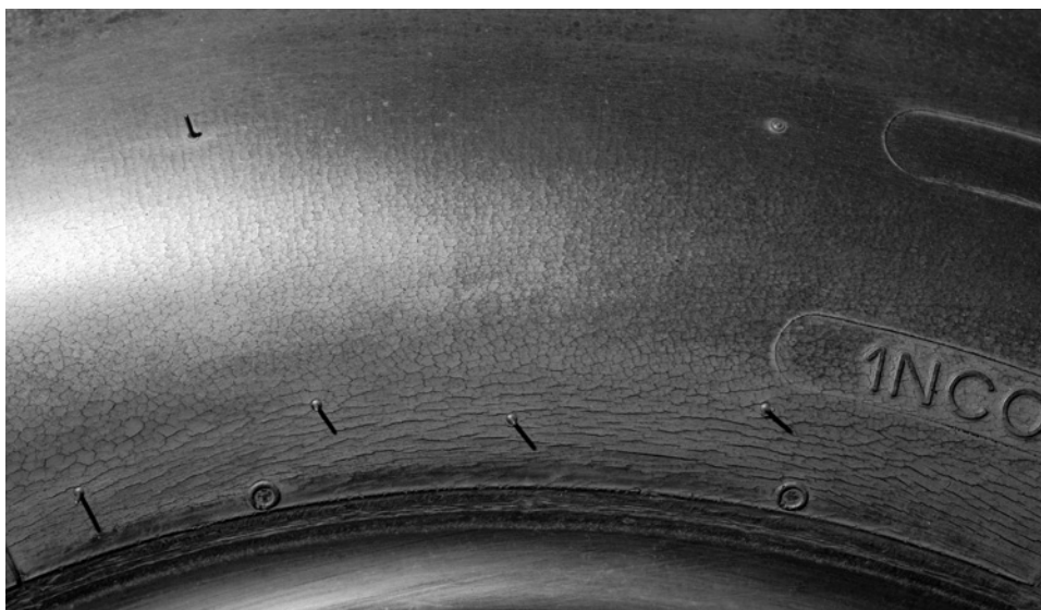
Figure 527. Sidewall Rubber Cracking
