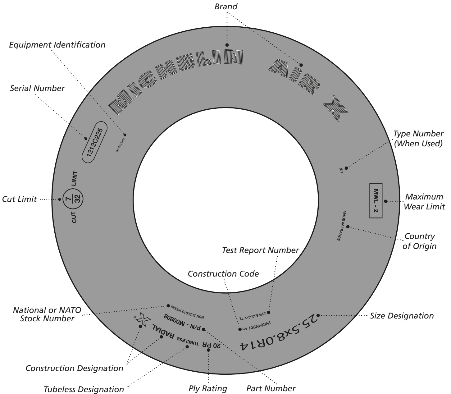
Figure 203. Typical Aircraft Tire Markings – Military Radial, US
