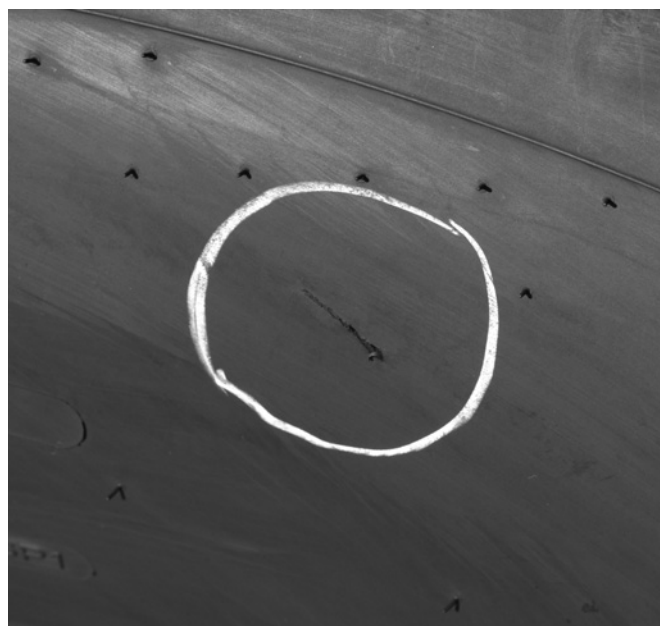
Figure 302. Damage From Contact With Sharp Object - Serviceable
