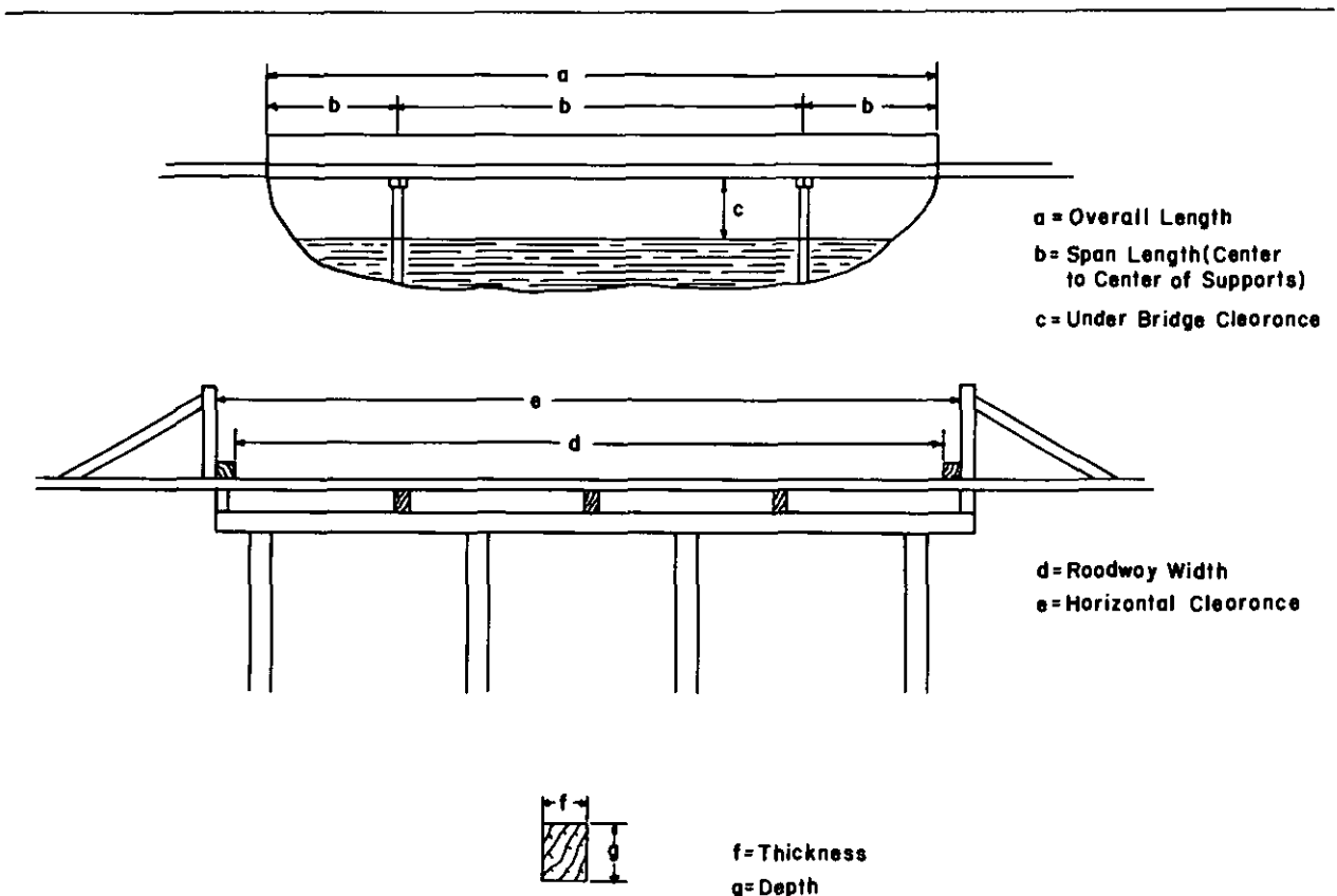
Figure 131. Typical timber cross section
