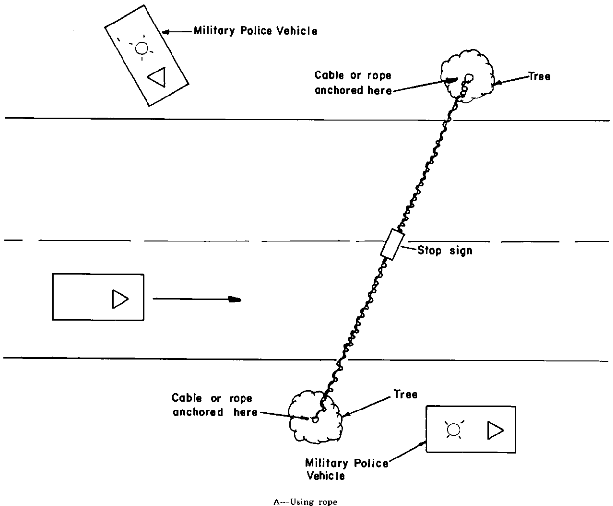
Figure 50. Example of a roadblock.
