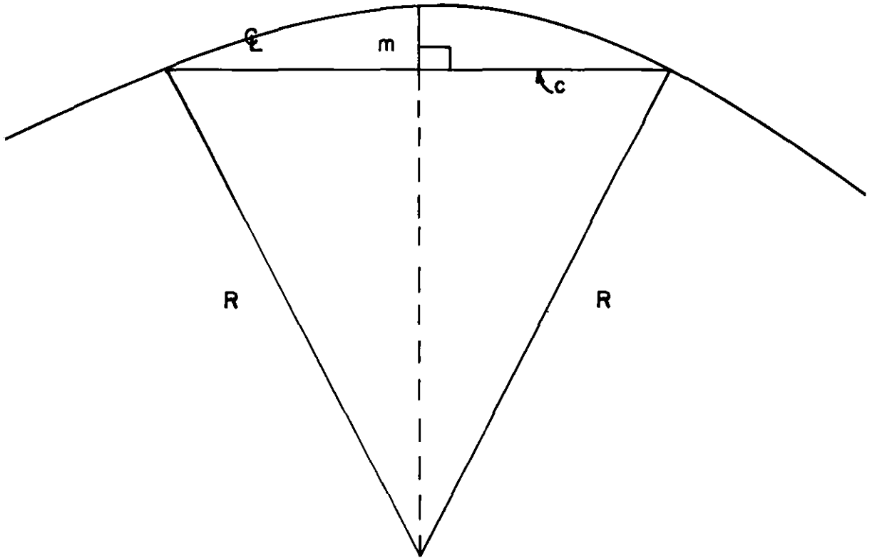
Figure 122. Measuring a curve using formula R=C^2/8m + m/2 .
