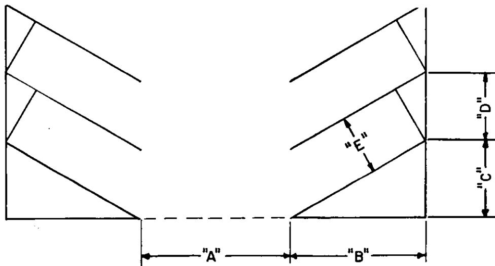
Figure 6. Dimensions for parking stalls.
