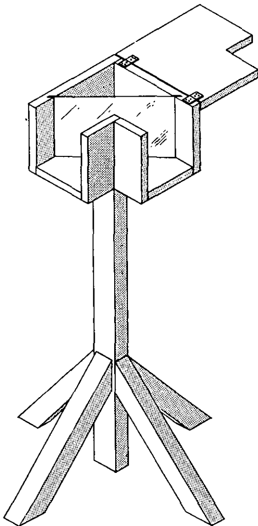
Figure 26. Mirror box.
