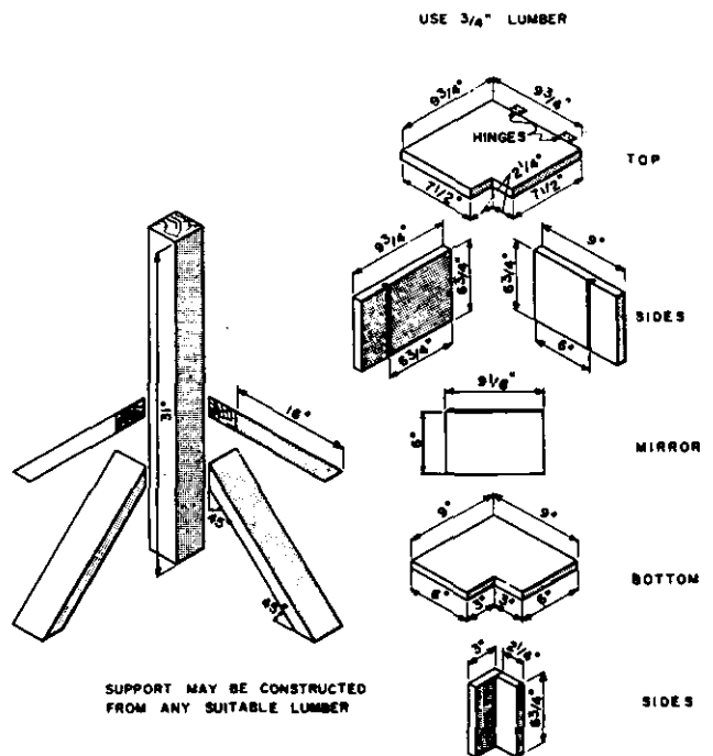
Figure 27. Dimensions of a mirror box.
