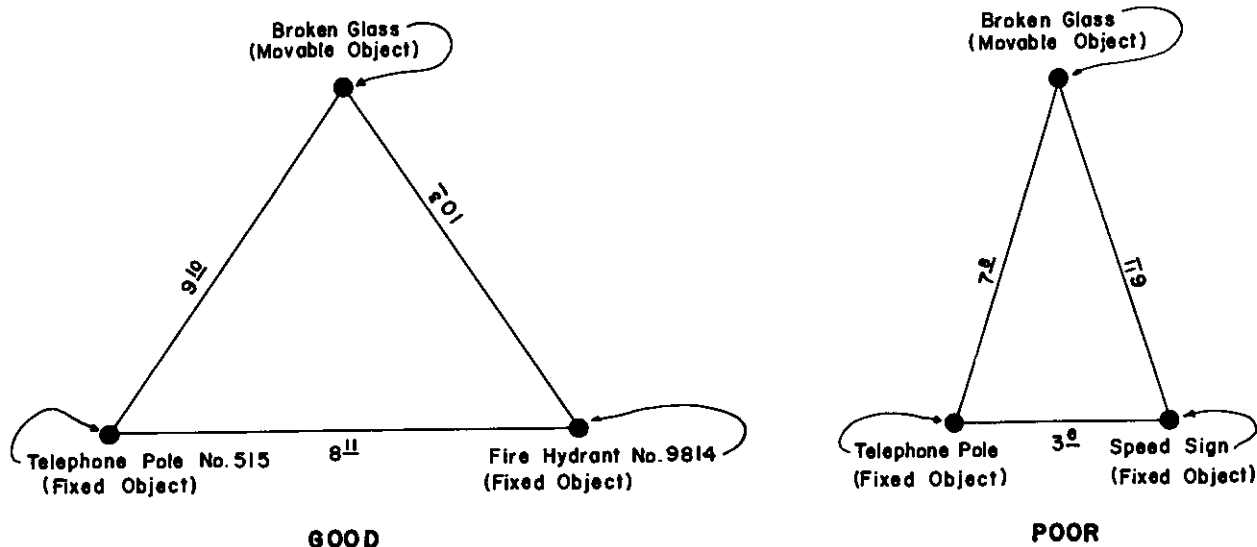
Figure 31. Example of triangles apex angle.
