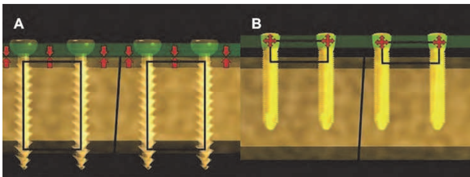
Fig. 15. Differences between distribution of the biomechanical load for standard plates (A) by comparison with LISS (B) and the bone implant interface.
