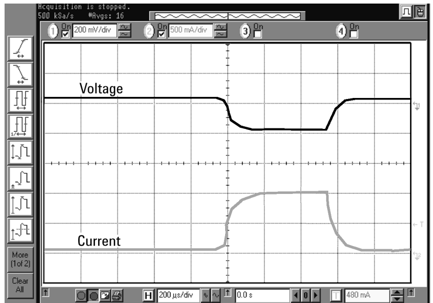
Figure 12. Actual NiMH battery voltage response with 230 milliohms of battery internal resistance
