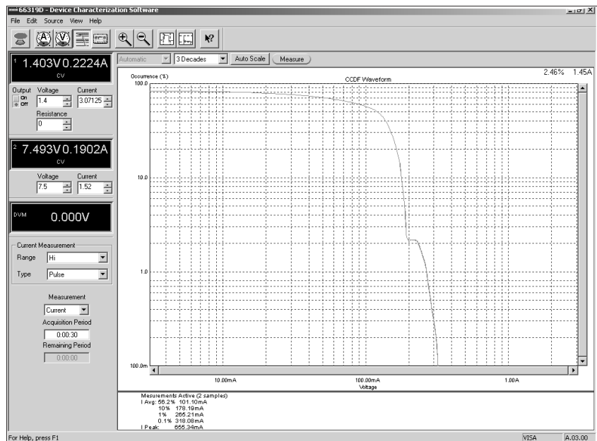
Figure 11. 14565B Device Characterization Software with Battery Drain Analysis displaying a CCDF chart (current vs % occurrence)
