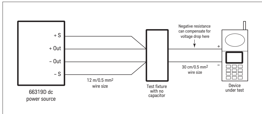
Figure 8. Using negative resistance to compensate for fixture/wiring resistance
