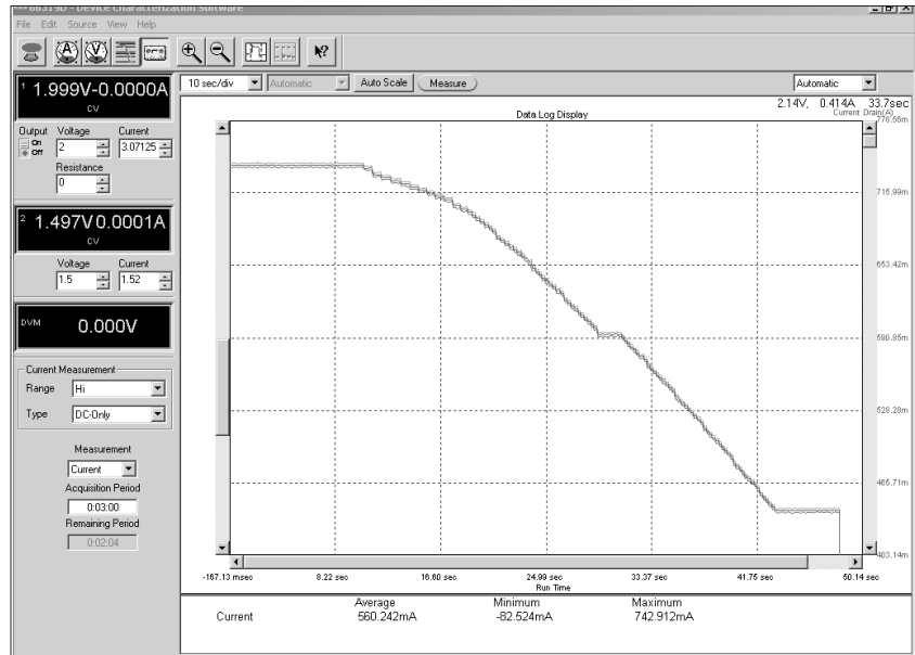
Figure 10. 14565B Device Characterization Software with Battery Drain Analysis displaying a long term data log
