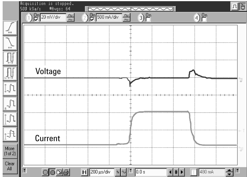
Figure 5. Actual output of 66319D with 6 meters of load leads and no fixture capacitor
