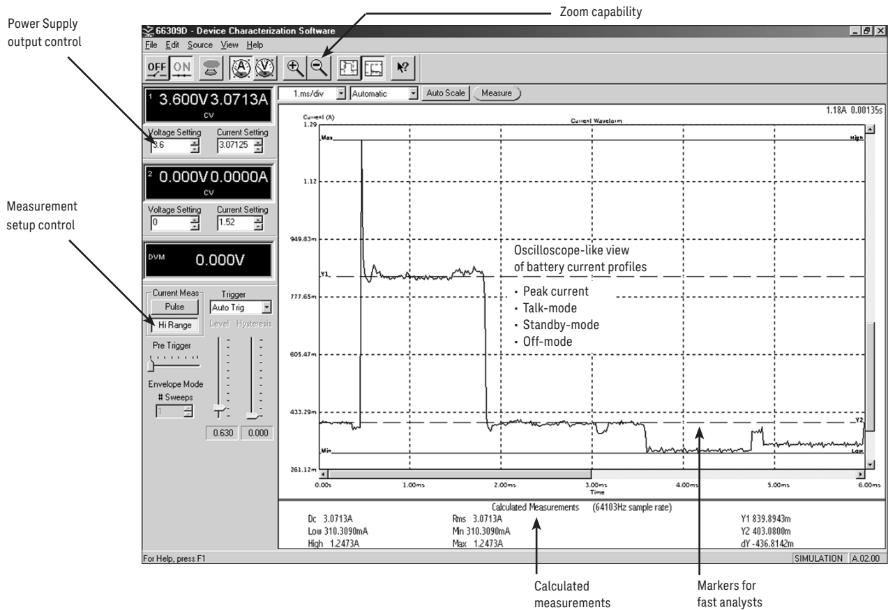
Figure 9. 14565B Device Characterization Software displaying GSM pulse current waveform
