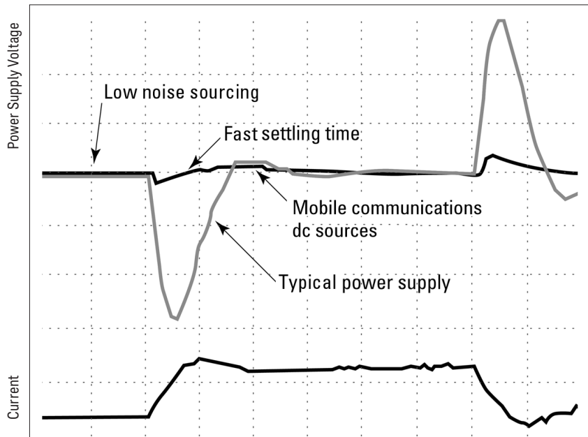
Figure 7. Settling time during GSM pulse: Comparison between general purpose power supply and Keysight Mobile Communications DC Source
