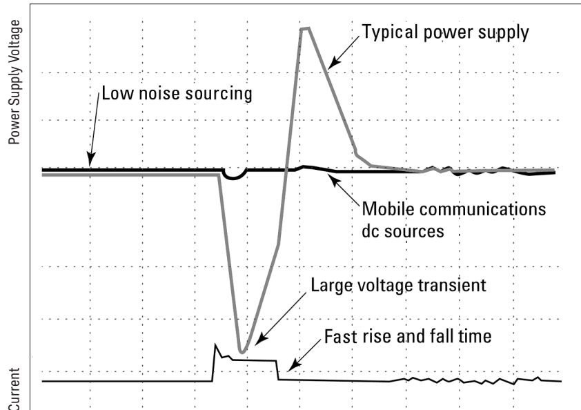
Figure 6. Transient response to typical GSM pulse: Comparison between general purpose power supply and Keysight Mobile Communications DC Source
