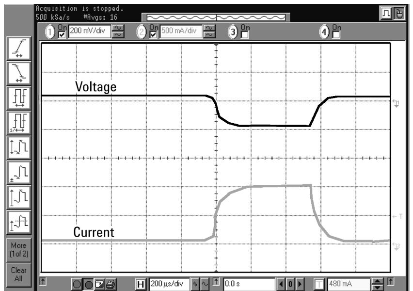
Figure 13. Actual output of the 66319D programming with 230 milliohms of output resistance
