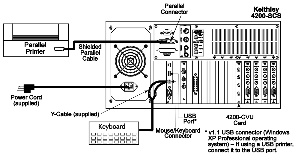
Figure 2: System connections
