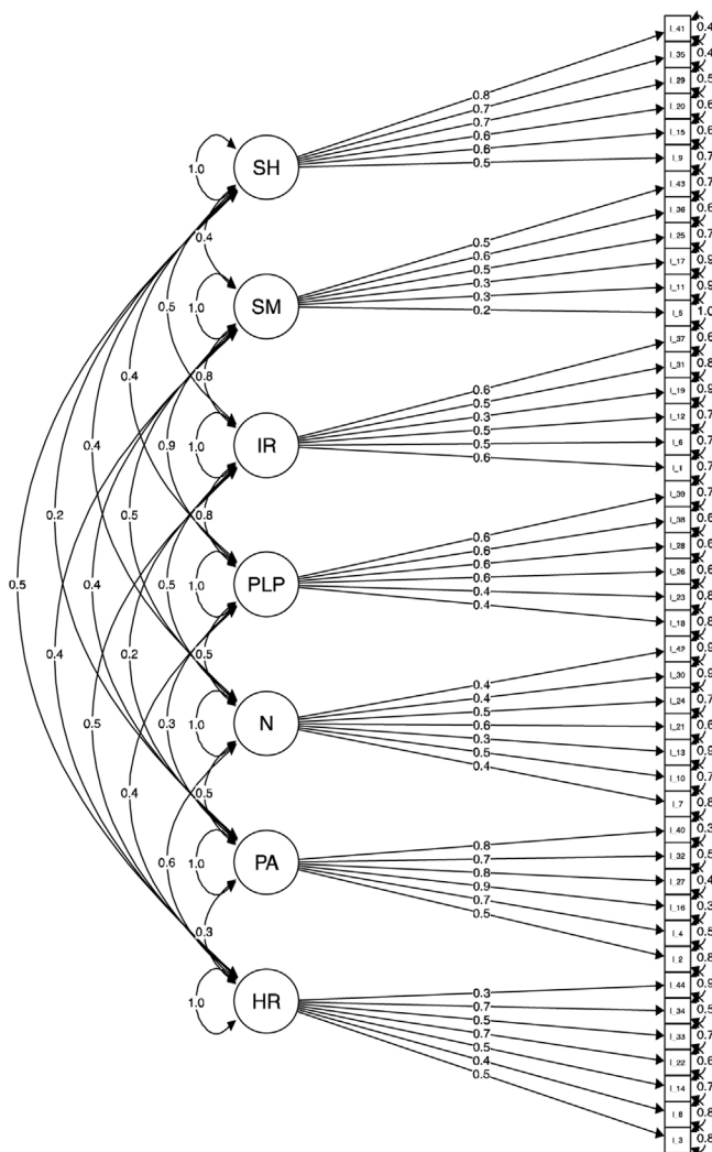
Figure 1 Items correlations properties ALPR2 in the Confirmatory factor Analysis.
