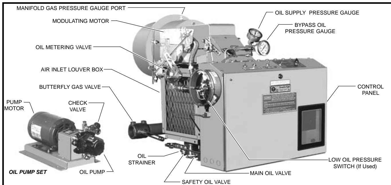
TYPICAL MODEL KS WITH E2-F7T GAS-OIL SYSTEM
