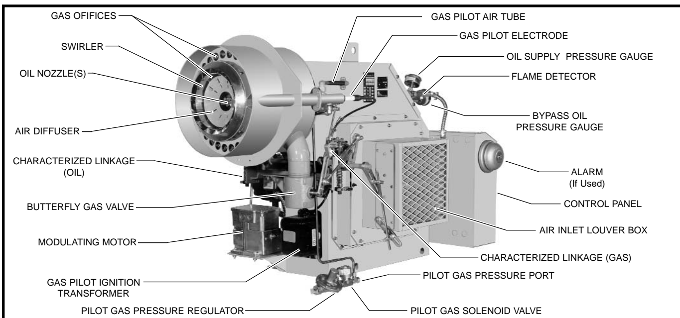
TYPICAL MODEL KS14 WITH E2-F7T GAS-OIL SYSTEM
