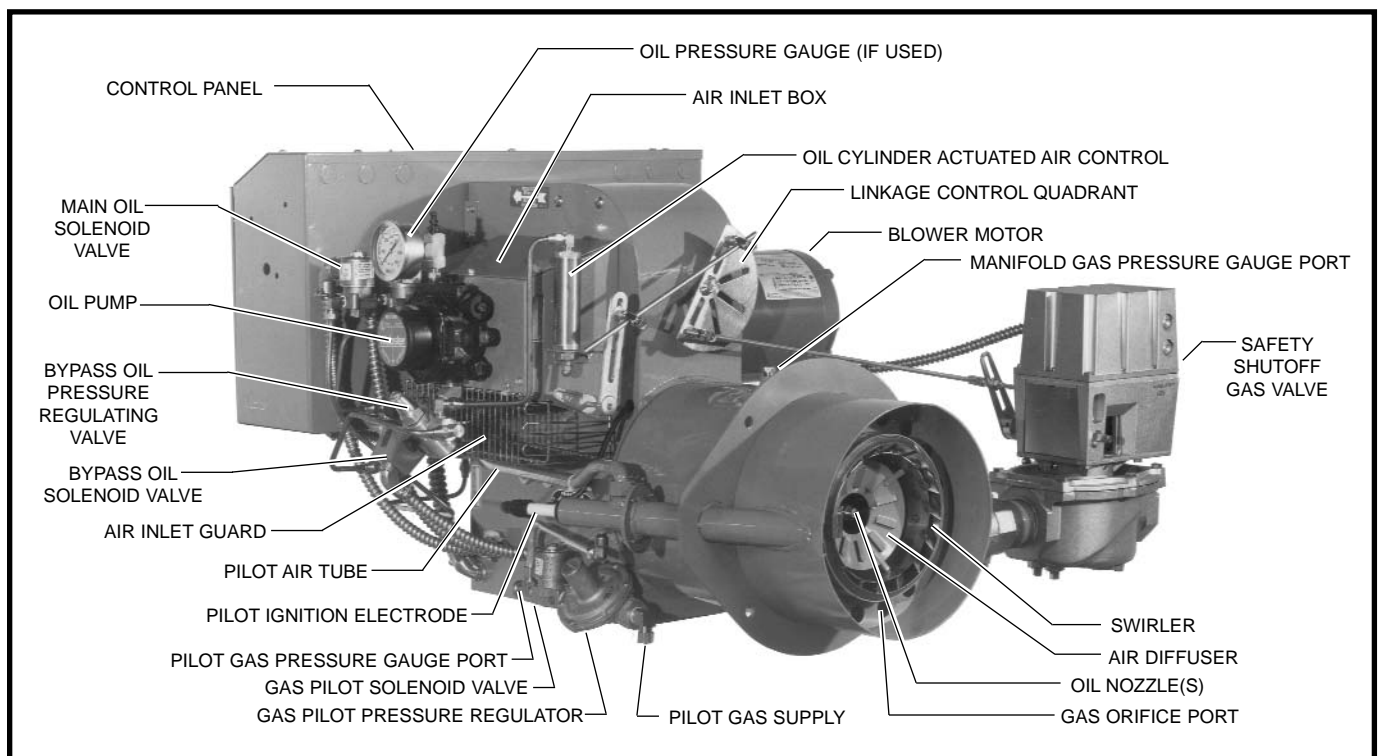
TYPICAL MODEL KR WITH H-F4S GAS-OIL SYSTEM
