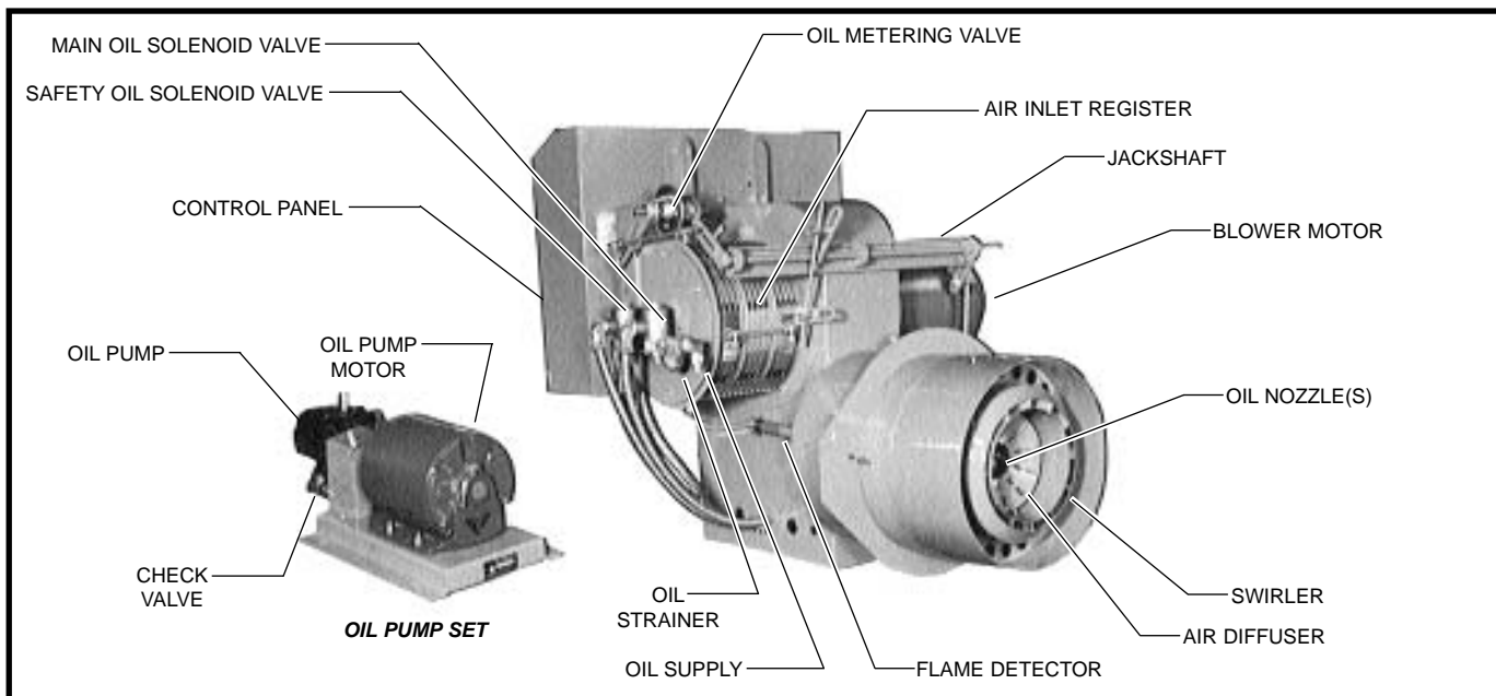
TYPICAL MODEL KR WITH F7T OIL SYSTEM
