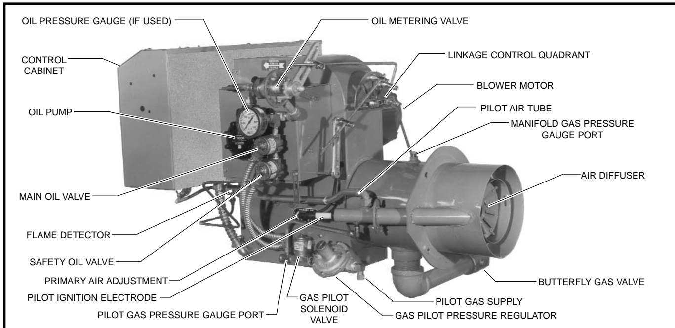
TYPICAL MODEL KR WITH E2-F6R GAS-OIL SYSTEM
