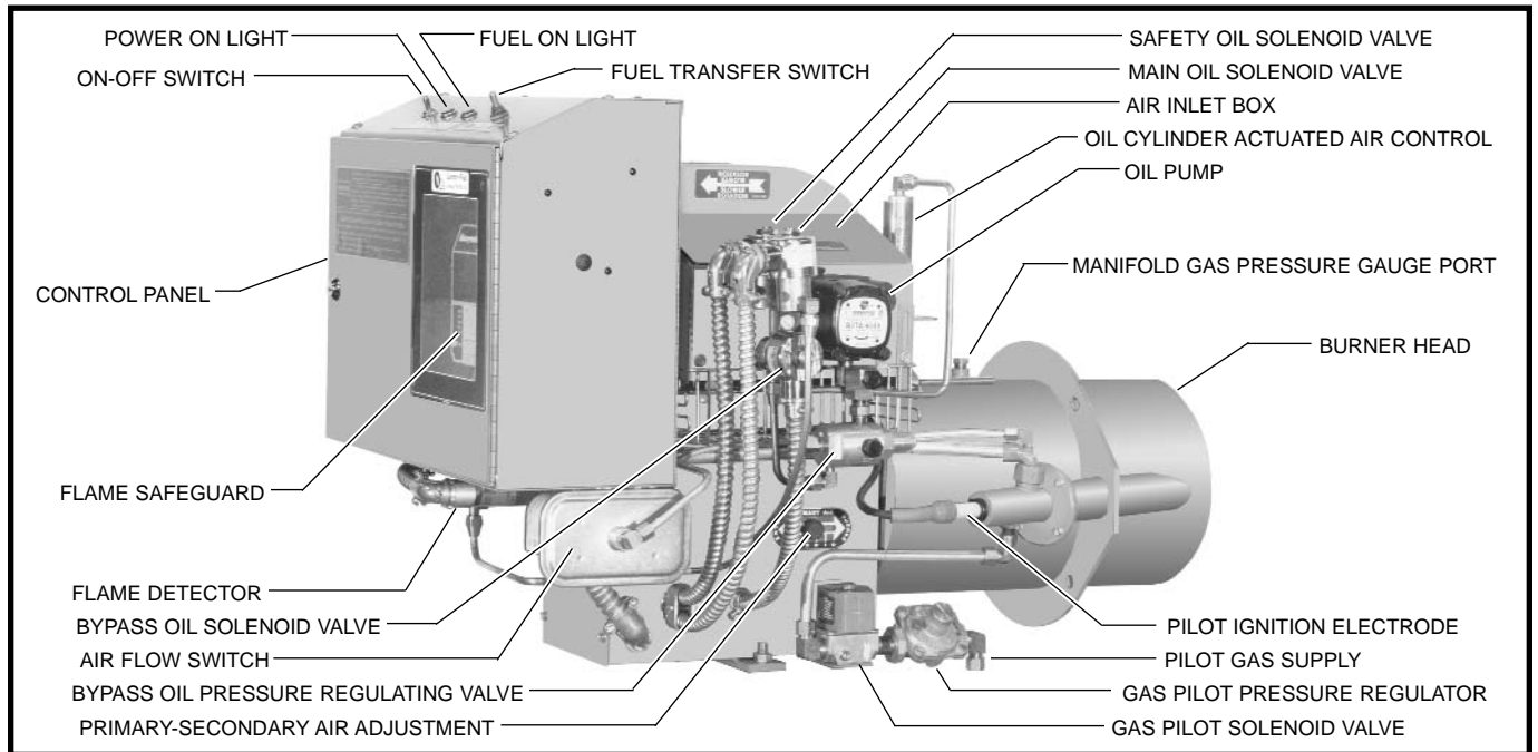
TYPICAL MODEL KR WITH B-F4B GAS-OIL SYSTEM
