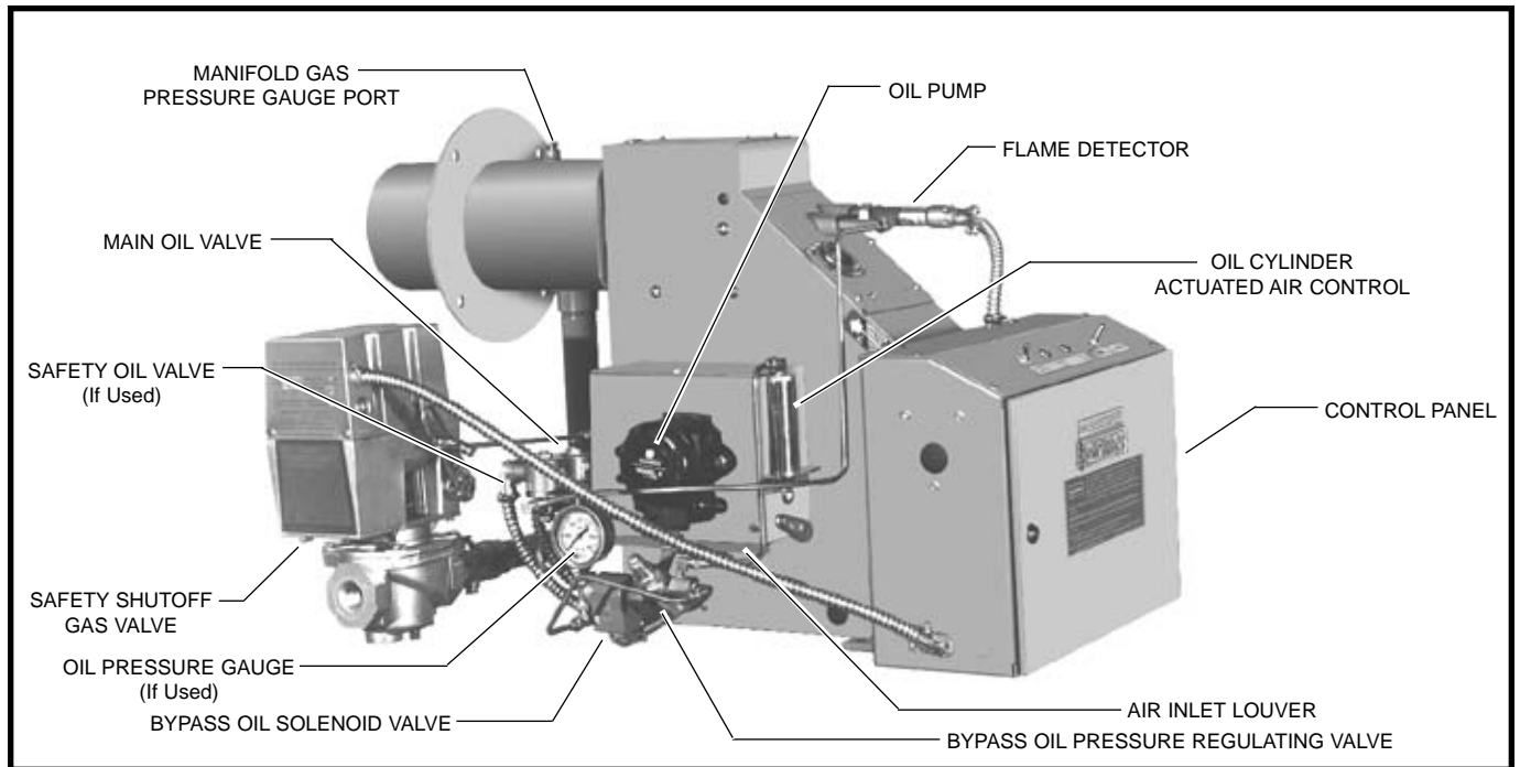
TYPICAL MODEL KS WITH H-F4S GAS-OIL SYSTEM
