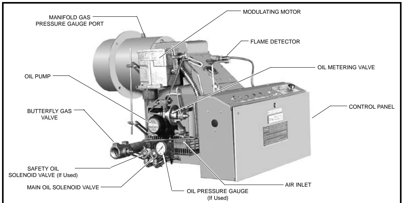
TYPICAL MODEL KS WITH E2-F6R GAS-OIL SYSTEM
