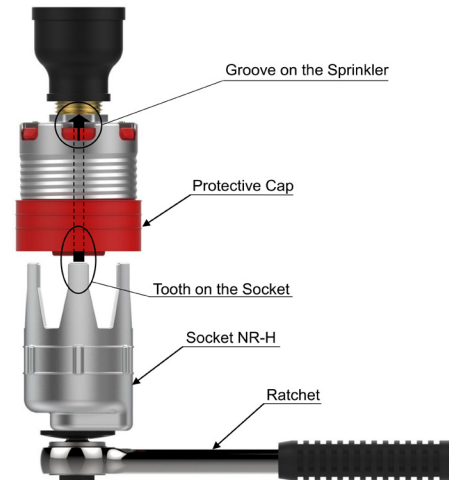
Figure 4: Ratchet & Socket
