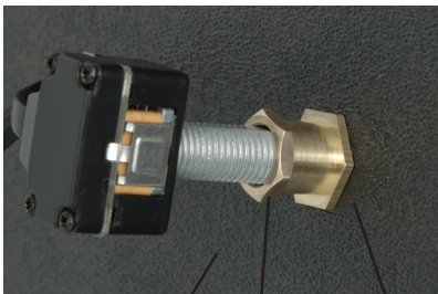
View behind dash Shaft Nut Collar Nut
