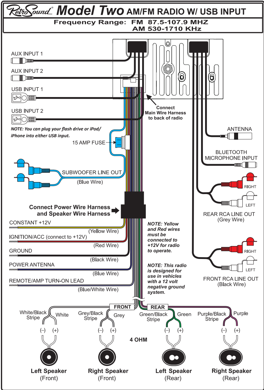
Figure 9 - Wiring Diagram
