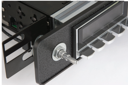
Figure 4 - Install Vehicle Specific Faceplate DO NOT OVERTIGHTEN SHAFT NUTS!!
