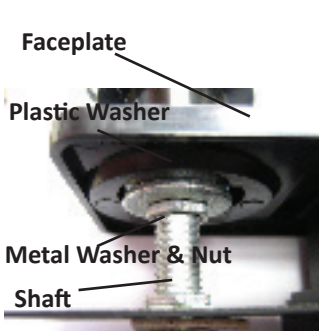
Nuts/washers installed between L bracket and faceplate
