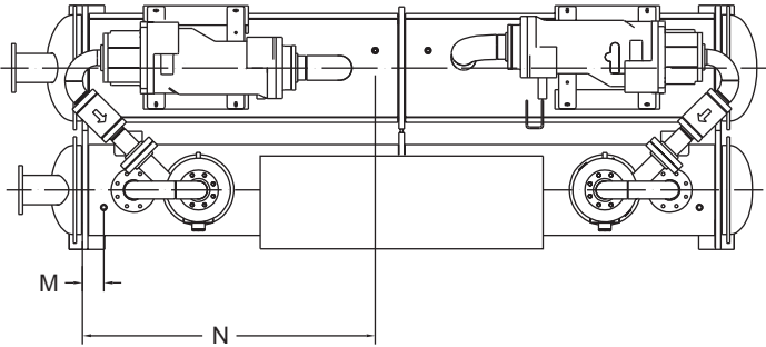
TOP VIEW - DUAL COMPRESSOR
