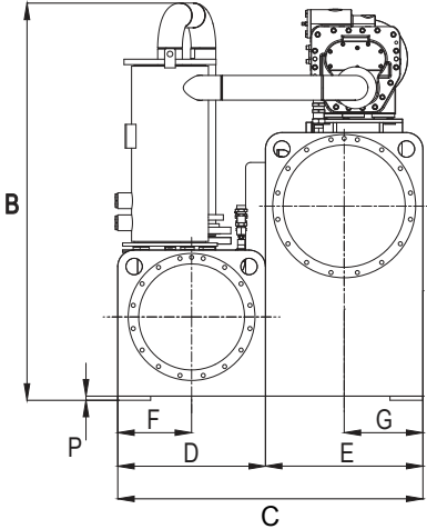
SIDE VIEW - BOTH
