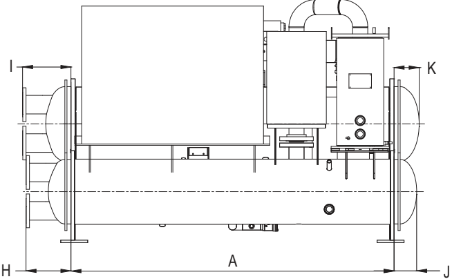
FRONT VIEW - DUAL COMPRESSOR
