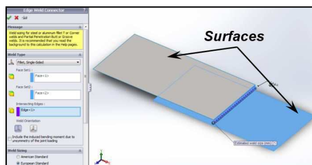
Figure 10: Edge weld connector for surfaces
