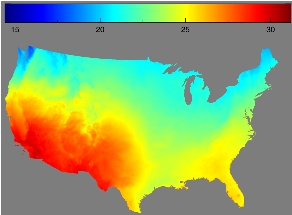
FIG. 12. The solar PV capacity factor map for the contiguous USA. The scale is from 14–33%. The capacity factor is for the individual panels described and tilted at latitude, tracking on one axis. Other solar PV panels will perform differently. It shows that the dynamic range over the US is not large. The Pacific North-West is particularly poor, and the South-West particularly good.
