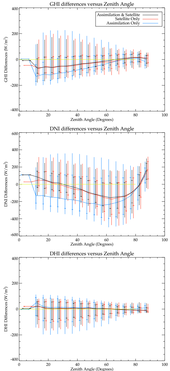
FIG. 4. The difference between the estimated irradiance and the measurement versus the zenith angle. The top panel is for GHI, the middle panel is for DNI, and the bottom panel is for DIF. The black is for regression scheme A, red is for scheme B, and blue is for C (similar to all other figures). The light green line designates the zero-line.
