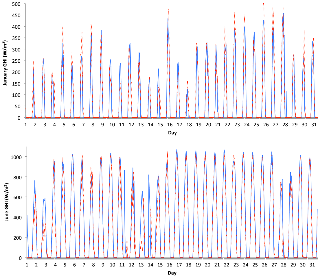
FIG. 5. Time series of measured (dashed red) and estimated (solid blue) GHI for Burns, OR. The top panel is for the 31 days from January 1 2006 and the bottom panel is for the 31 days following June 1 2006. The panels show high correlation between the estimated and the measured.
