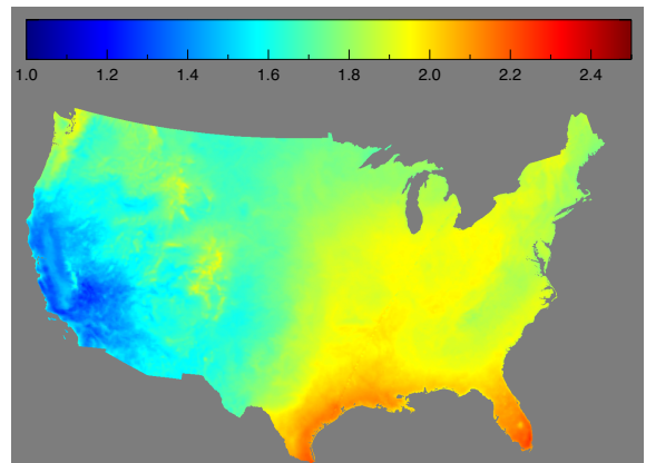
FIG. 11. The average estimated DIF in kWh/m 2 /day for the contiguous USA over the three year period of 2006–2008 (the range is different to figs 9 and 10). The Gulf Coast has the most DIF resource, the South West has the least DIF, and in general the East has more DIF than the West. All boundaries have been removed to display the detail of the data.
