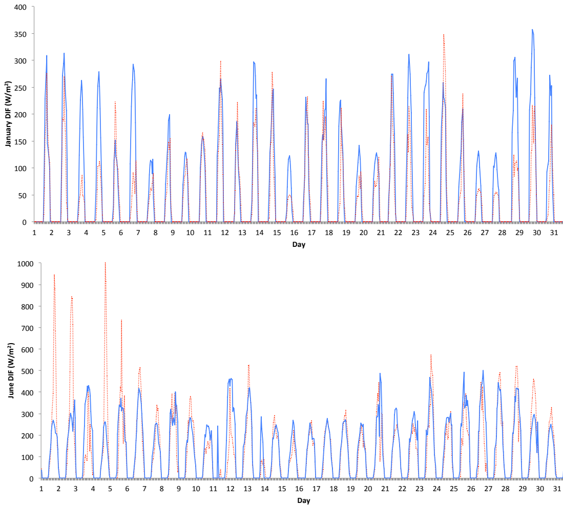
FIG. 7. Time series of measured (dashed red) and estimated (solid blue) DIF for Elizabeth, NC. The top panel is for the 31 days from January 1 2006 and the bottom panel is for the 31 days following June 1 2006. The panels show high correlation between the estimated and the measured.
