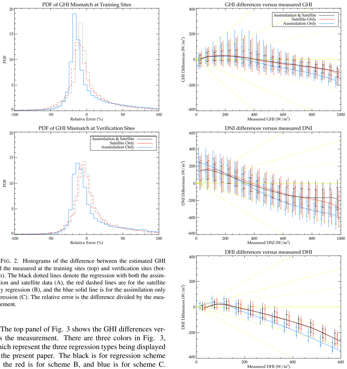
FIG. 3. The difference between the estimated irradiance and the measurement versus the measured irradiance. The top panel is for GHI, the middle panel is for DNI, and the bottom panel is for DIF. The black is for regression scheme A, red is for scheme B, and blue is for C (similar to all other figures). The light green line designates the zero-line.
