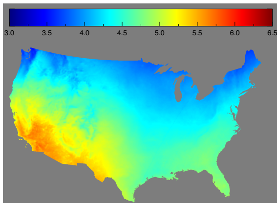
FIG. 9. The average estimated GHI in kWh/m 2 /day for the contiguous USA over the three year period of 2006–2008. The South West has the greatest resource while the North West and East have the least. All boundaries have been removed to display the detail of the data.
