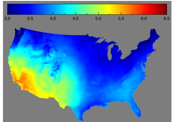
FIG. 10. The average estimated DNI in kWh/m 2 /day for the contiguous USA over the three year period of 2006–2008. The South West is the best resource area whereas the rest of the USA is much poorer. All boundaries have been removed to display the detail of the data.
