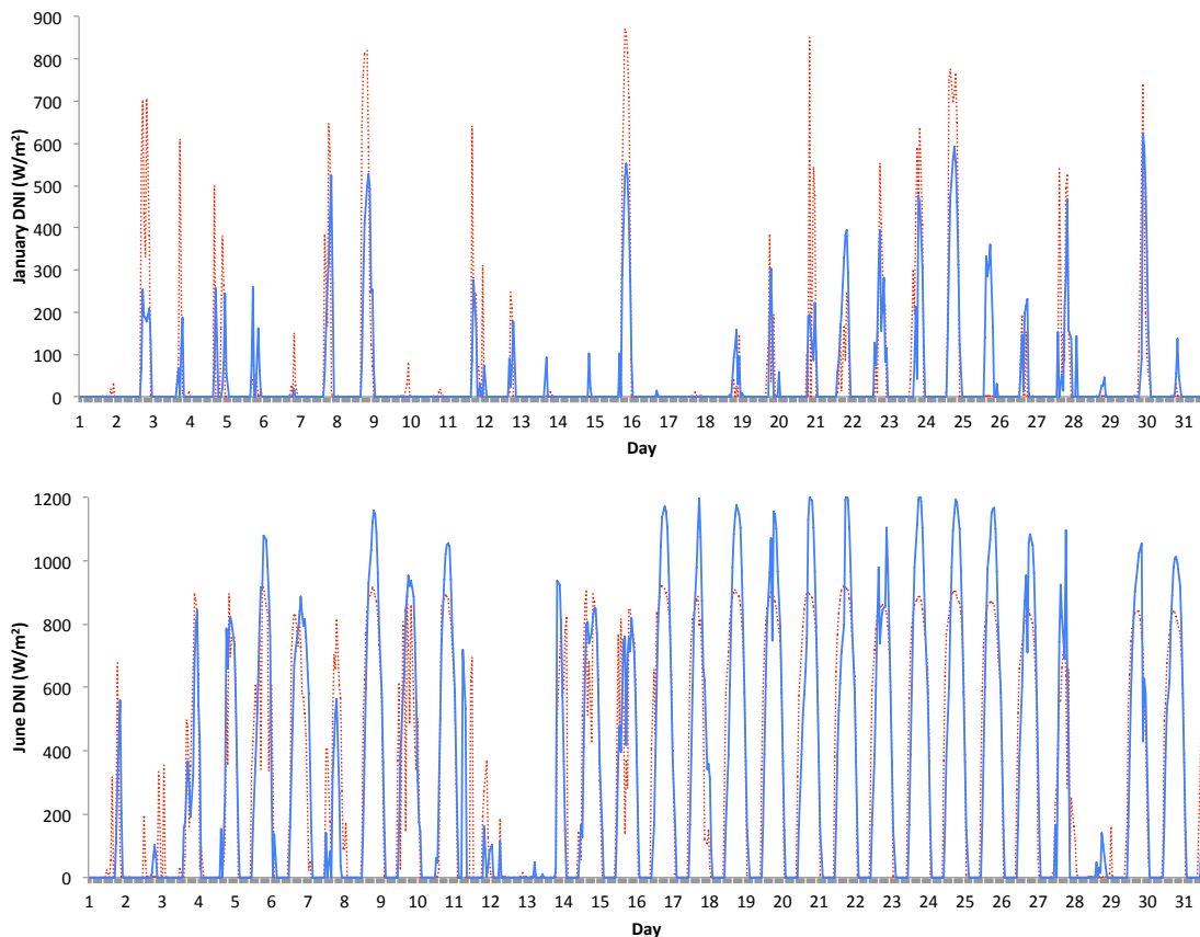
FIG. 6. Time series of measured (dashed red) and estimated (solid blue) DNI for Hermiston, OR. The top panel is for the 31 days from January 1 2006 and the bottom panel is for the 31 days following June 1 2006. The panels show high correlation between the estimated and the measured.
