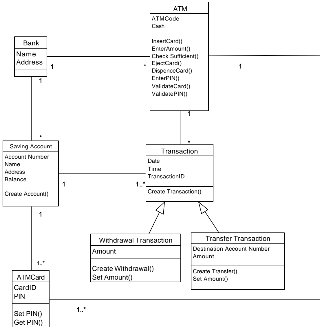
Gambar 3.13 Class Diagram
