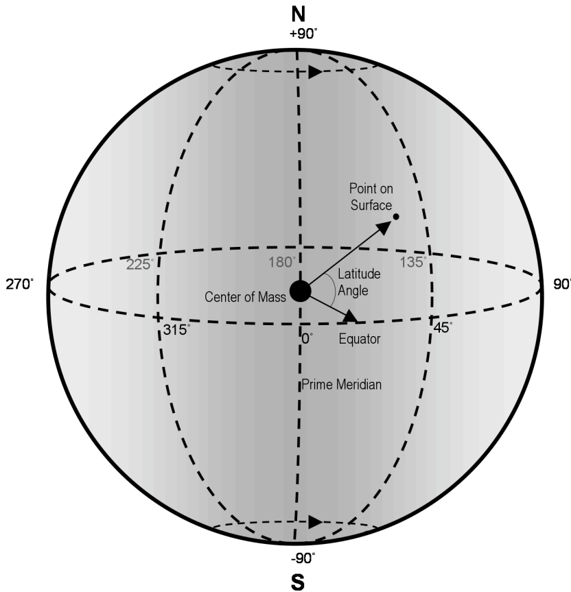
Figure 2-20. Planetocentric coordinates are expressed as right-handed coordinates with the origin at the center of mass of the body (from LRO Working Group, 2007).
