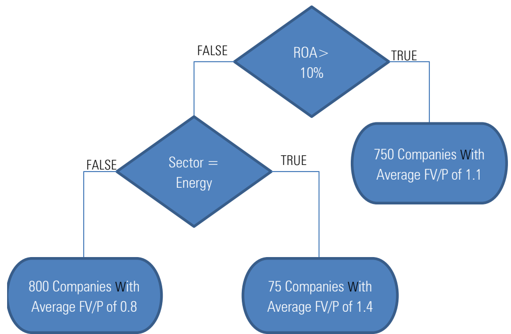
Exhibit 9 Sample Representation of a Regression Tree With Dummy Data
