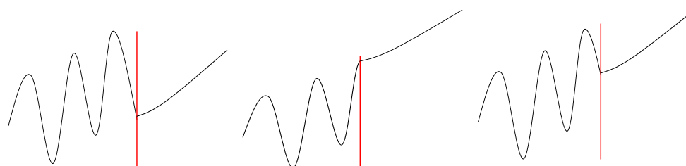
Exhibit 11 Choosing an EBI Forecast in the Last Year of Stage I
