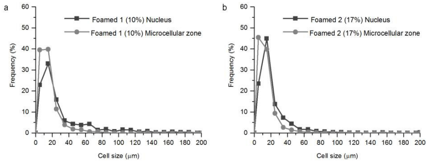
Fig. 4. Frequency cell size distribution in Ø = 5 mm section of bar A with (a) 10% of weight reduction; (b) 17% of weight reduction.
