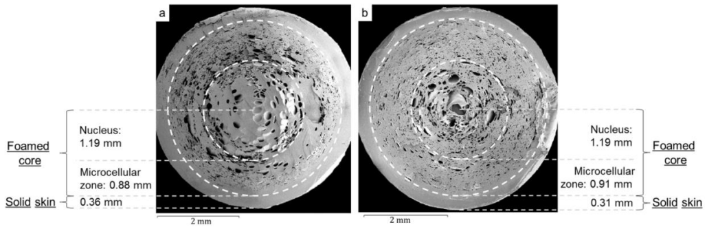
Fig. 3. SEM micrographs of Ø = 5 mm section and morphology areas of bar A with (a) 10% of weight reduction; (b) 17% of weight reduction.
