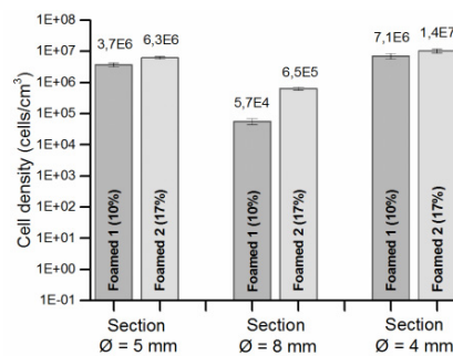
Fig. 7. Cell density in foamed bars.
