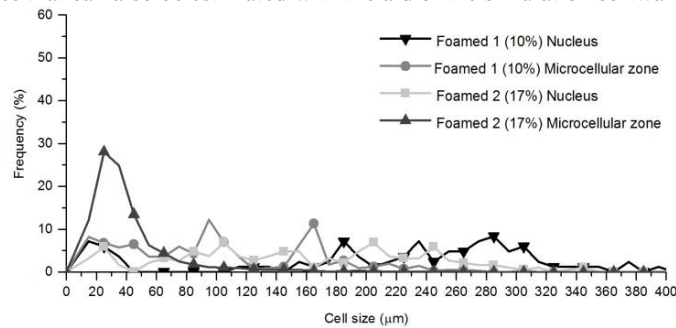
Fig. 6. Frequency cell size distribution in \varnothing = 8 mm section of bar A.
