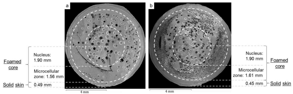
Fig. 5. SEM micrographs of Ø = 8 mm section and morphology areas of bar A with (a) 10% of weight reduction; (b) 17% of weight reduction.
