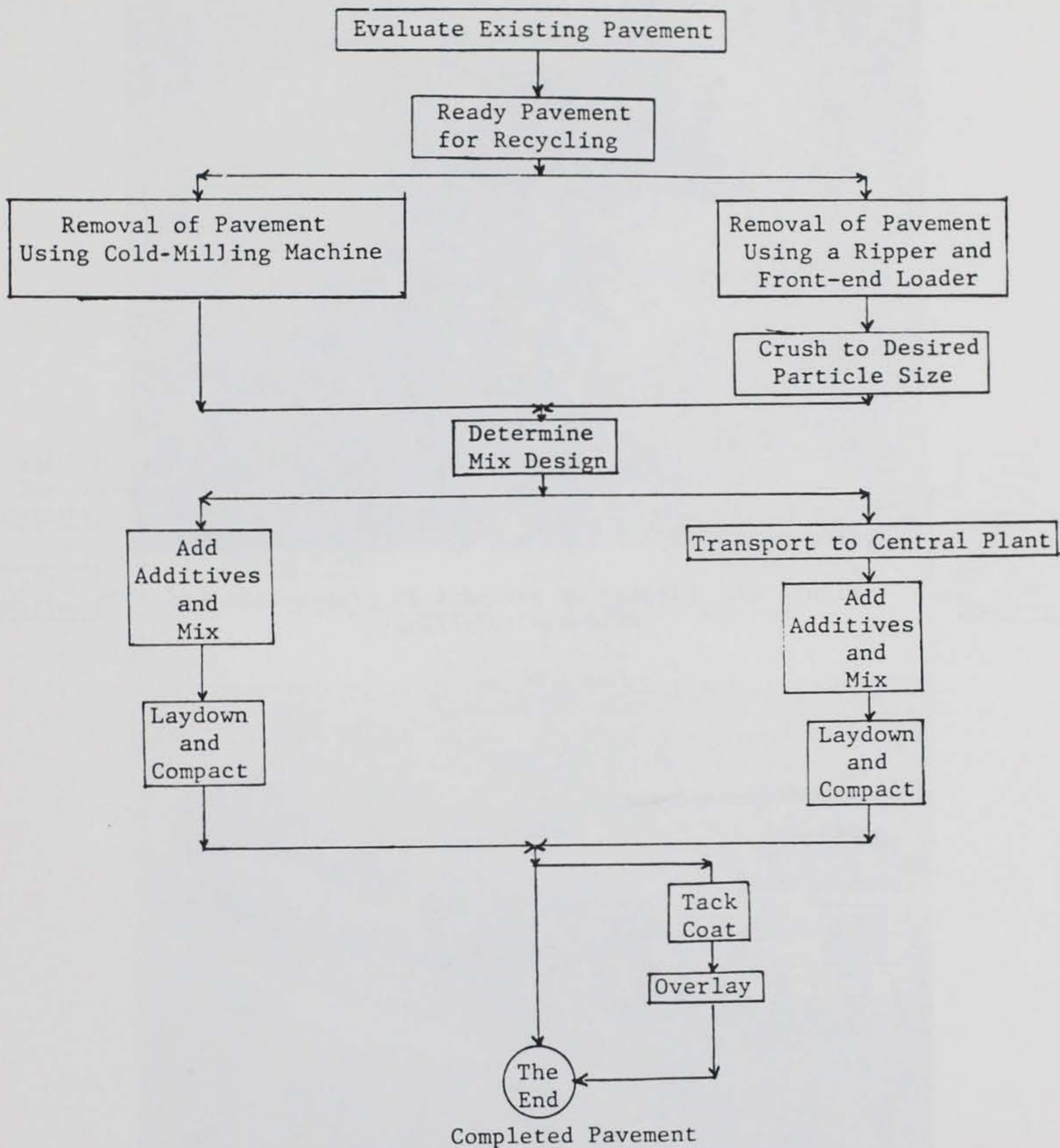
Figure 12. Cold-mix recycling flow diagram
