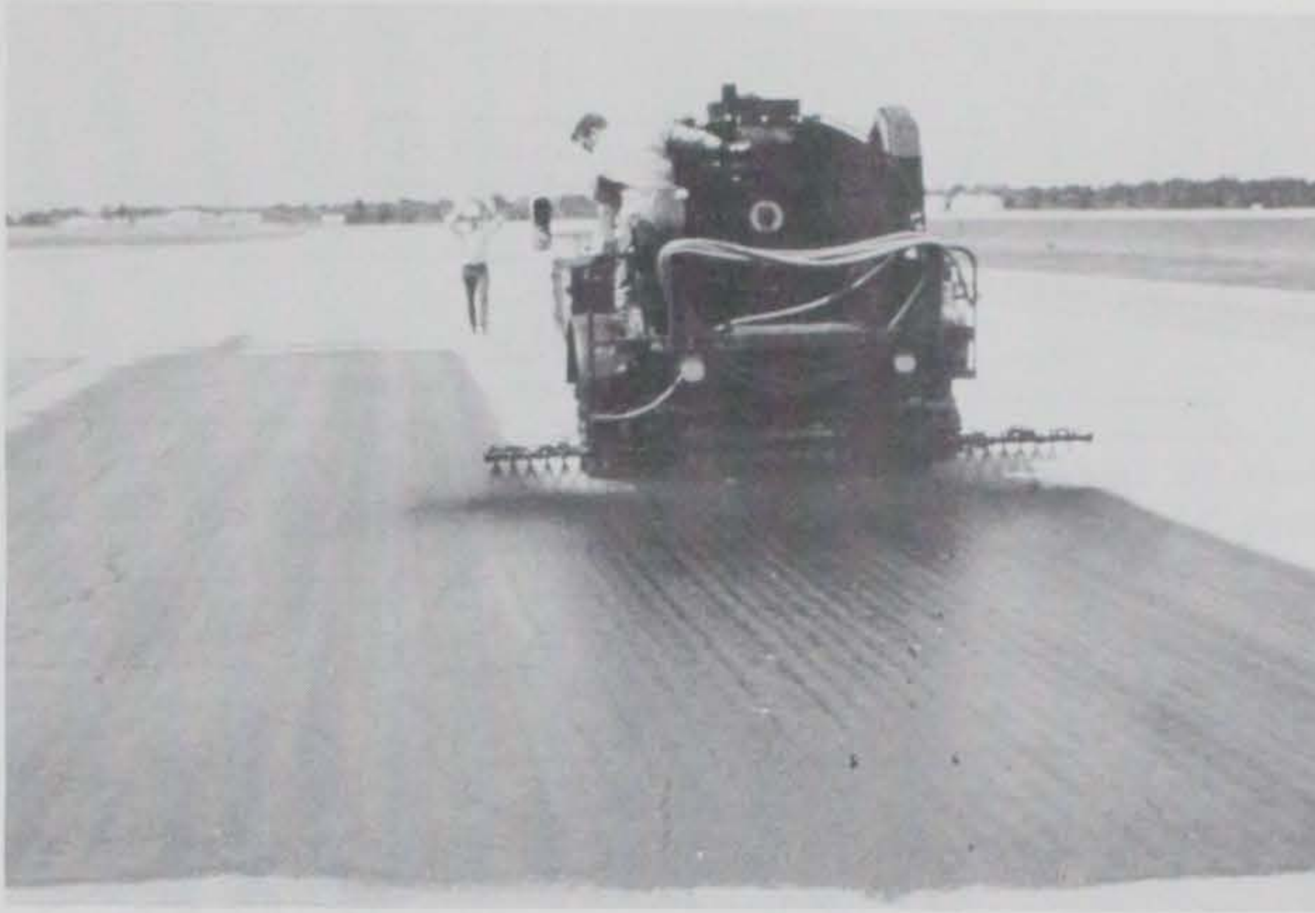
Figure 9. Asphalt distributor used to spray a rejuvenator
