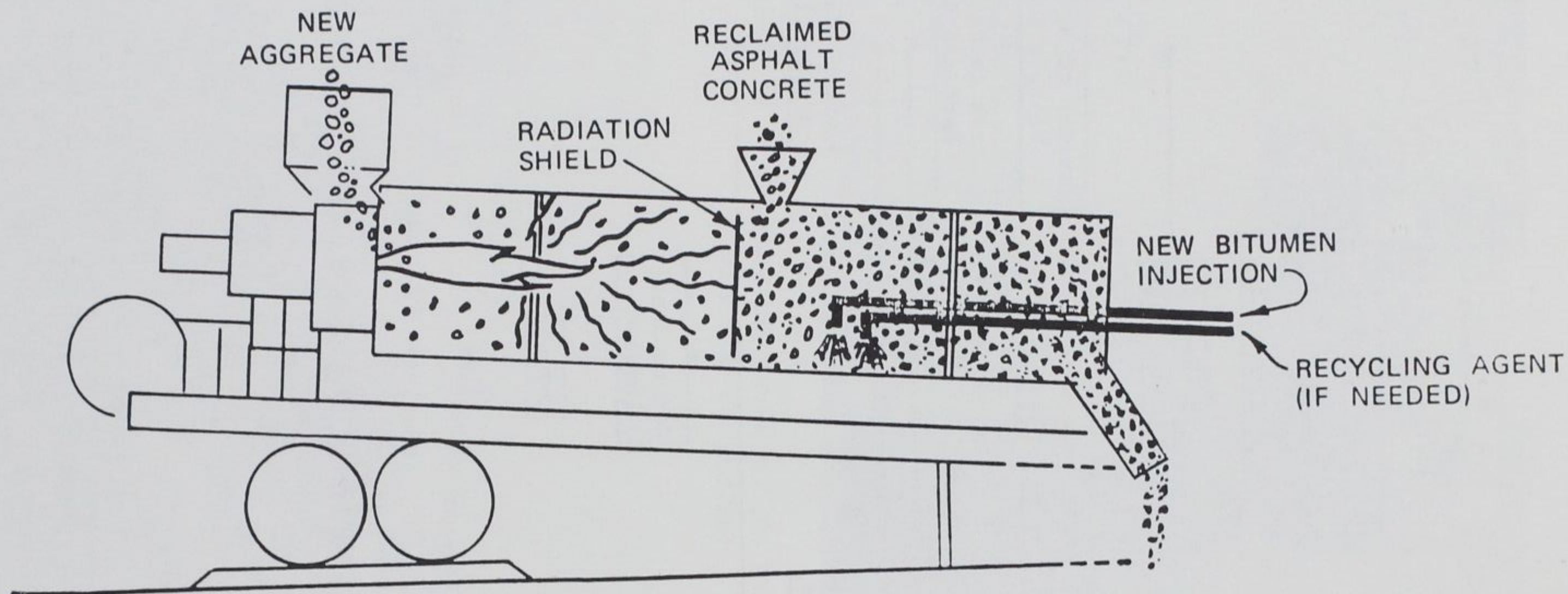
Figure 16. Drum plant
