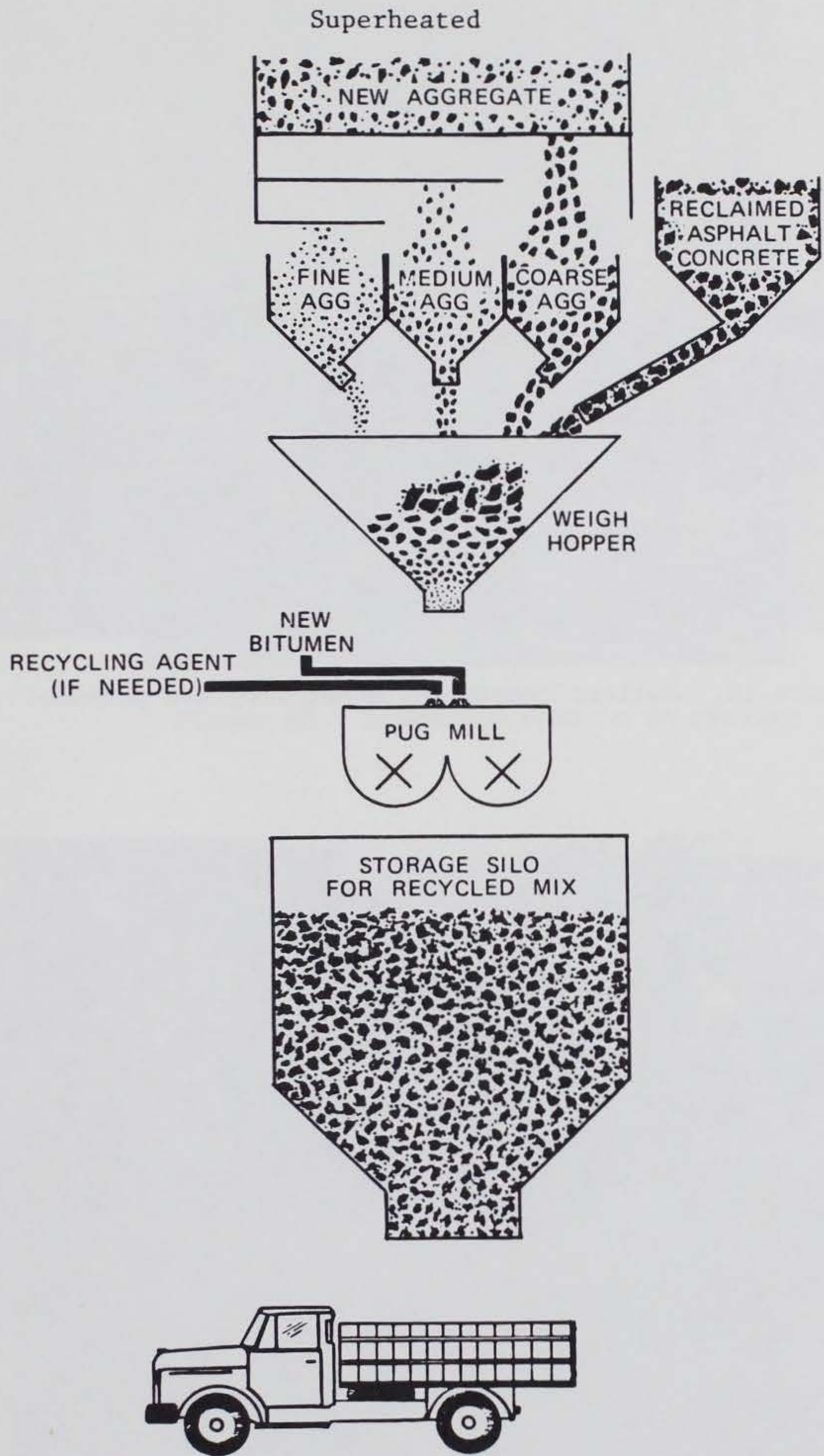
Figure 17. Batch plant
