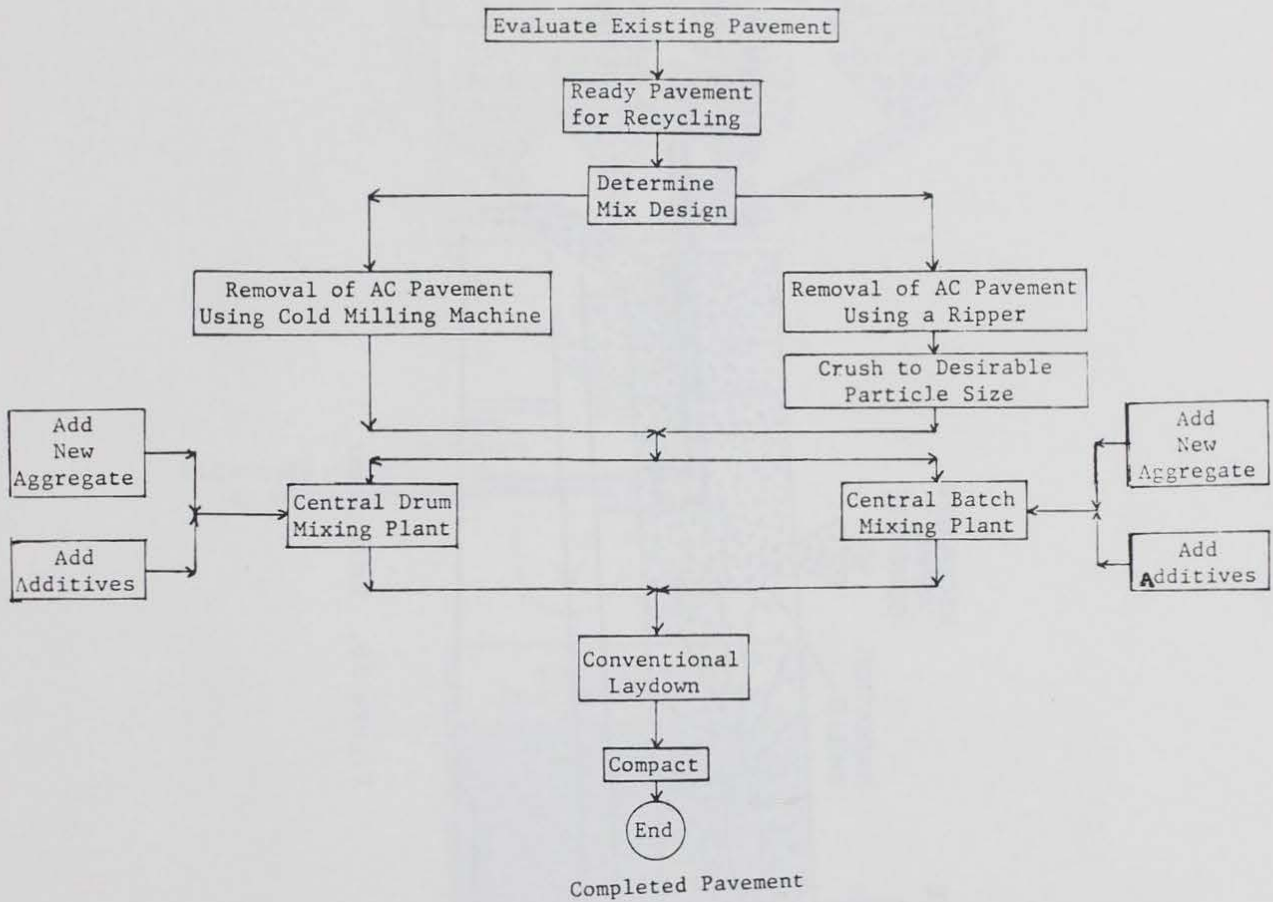
Figure 15. Hot-mix recycling flow diagram
