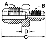
REDUCING UNION
