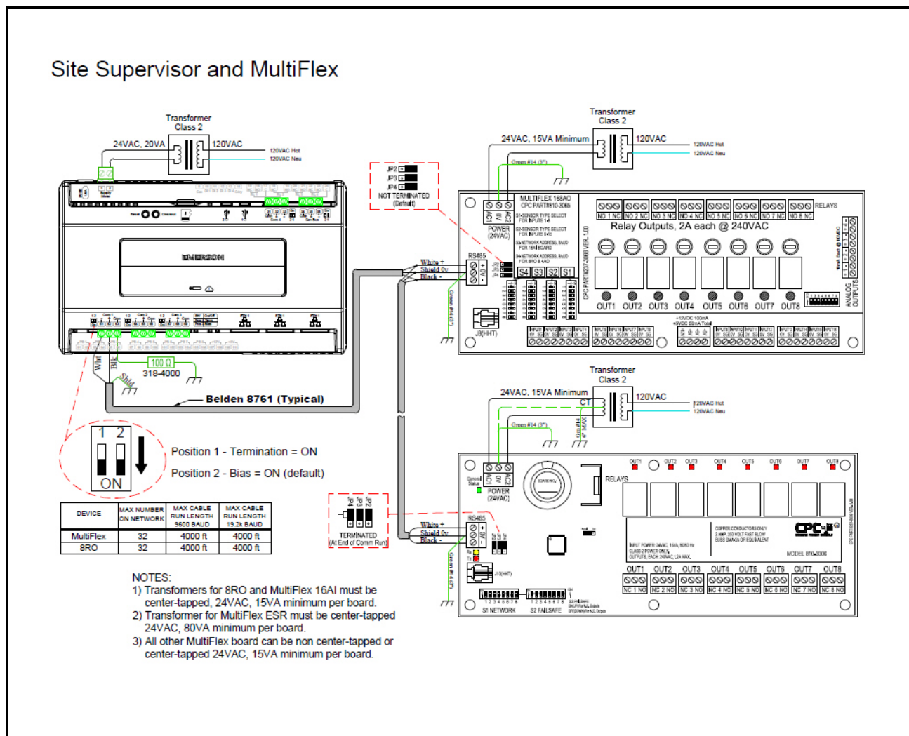
Figure 7-1 - Site Supervisor Wiring
