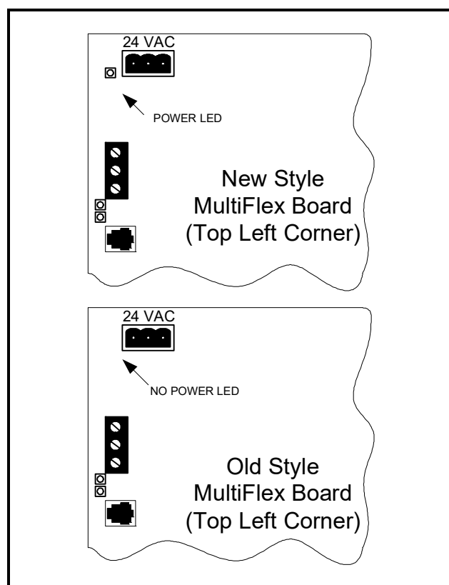
Figure 2-5 - New-Style vs. Old-Style MultiFlex Board
