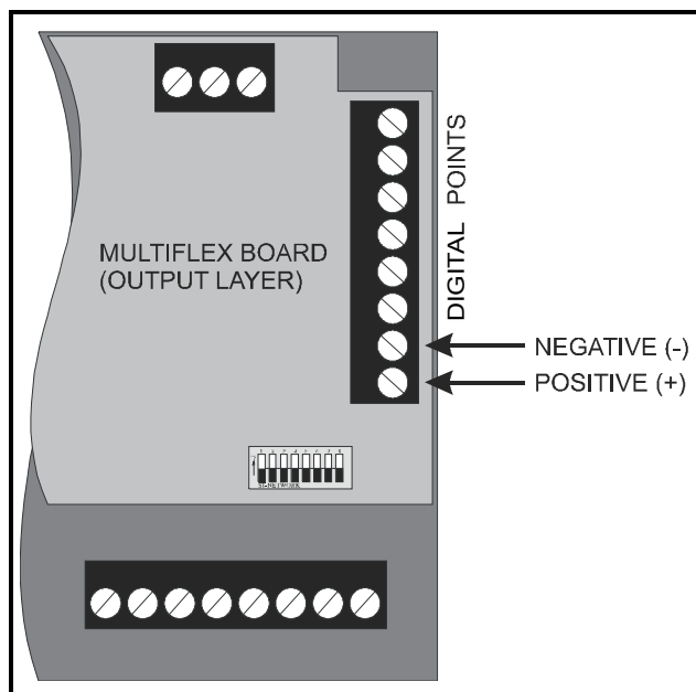
Figure 4-8 - MultiFlex Digital Points
