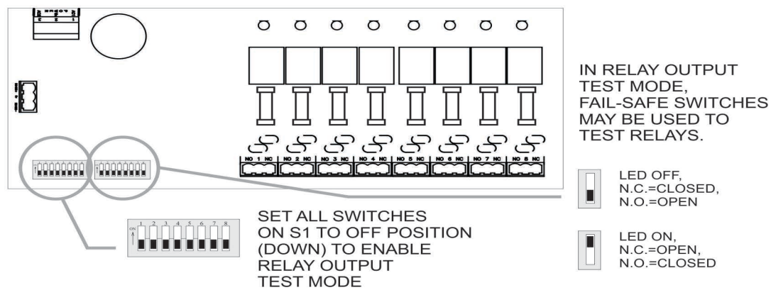
Figure 8-1 - Relay Output Test Modes
