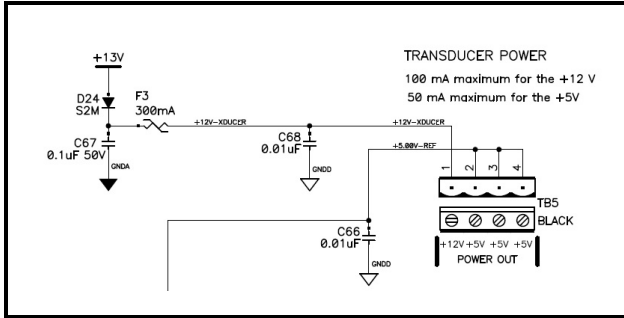
Figure 4-5 - MultiFlex Voltage Output View
