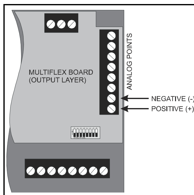
Figure 4-7 - MultiFlex Analog Points
