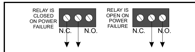
Figure 4-6 - Form C Contact Wiring
