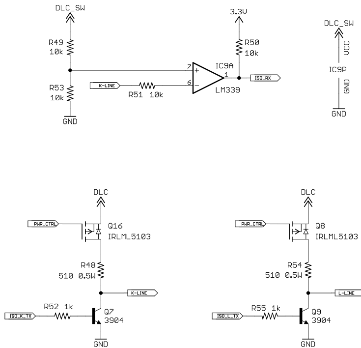
Figure 10 – ISO 9141/ISO 14230 Transceiver
