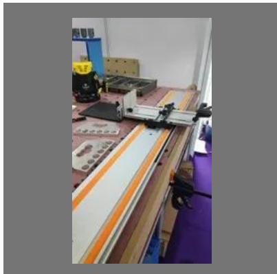
Manual Panel Saw
