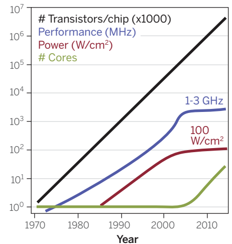
Fig. 4. Detailed look at Moore’s law for high-performance transistors. Approximate plot of various metrics in high-performance microprocessors over the past >40 years [lines are approximate fits to actual data, see (3)]. The oft-quoted version of Moore’s law is the number of transistors per chip (black line), but key trade-offs in chip performance (clock frequency, blue curve) have been made since the early 2000s because of the power density (red curve) reaching a physical limit of \sim 100 W/cm 2 . Continued Moore’s law scaling of high-performance transistors has been sustainable only by multicore architectures (green curve)—and the associated “dark silicon”—for the past decade.
