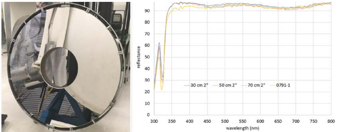
Fig. 3. Left: The MCAT mirror with its new enhanced, protected silver coating. Right: The reflectance curves, including: YELLOW: the originally proposed coating, BLUE, RED, GREY – actual final reflectivity as measured from witness samples that were coated in the chamber with the MCAT mirror. The throughput demonstrates the superior and uniform coating across the entire surface.
