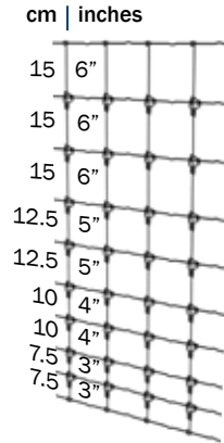
10/110/15 Intensive goat
