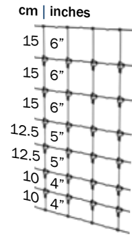
8/90/15 Intensive boundary
