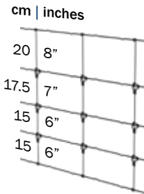
5/70/30 Sheep only
