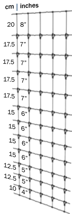
13/190/15 Intensive boundary/Emu
