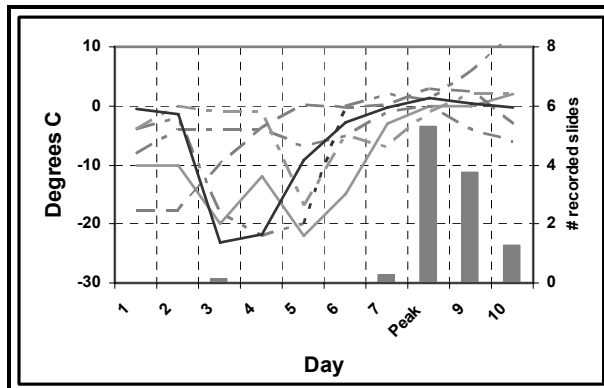
Figure 18: Graph depicting daily maximum temperatures (Pike Creek SNOTEL) clustering near 0°C on day of peak avalanche activity for 6 significant avalanche cycles 1996-2004
