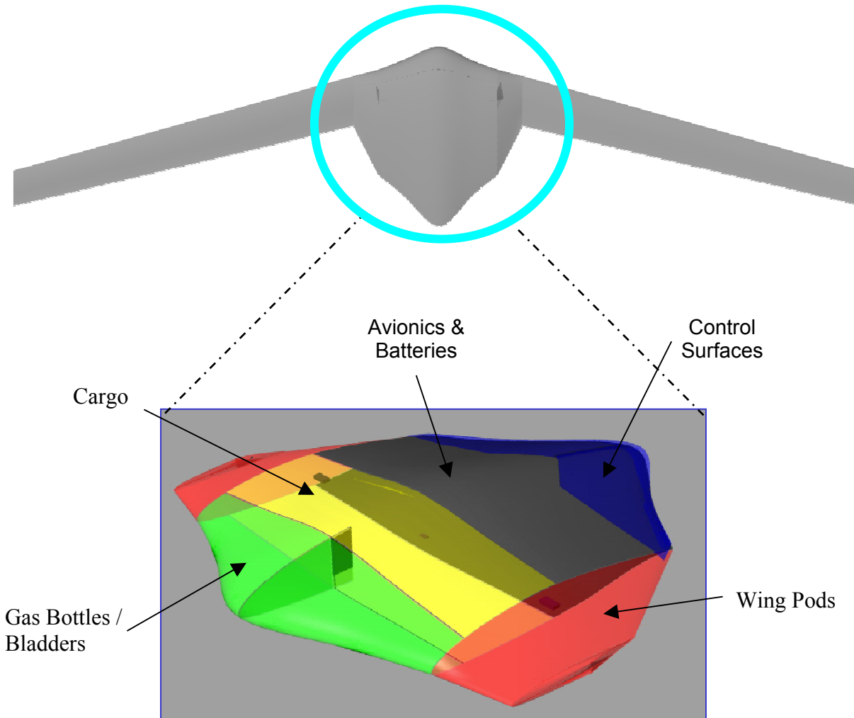
Figure 20 Centerbody Configuration
