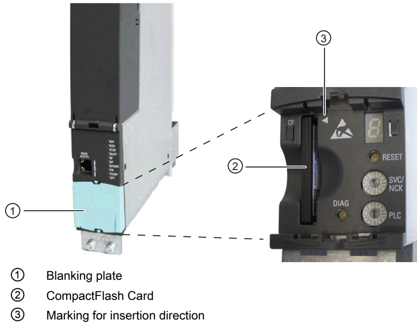
Figure 10-2 Inserting the CompactFlash card
