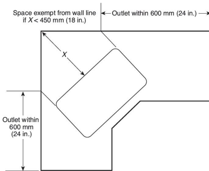
Range, counter-mounted cooking unit mounted in corner
