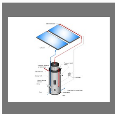
Hotel Tank Heating System
