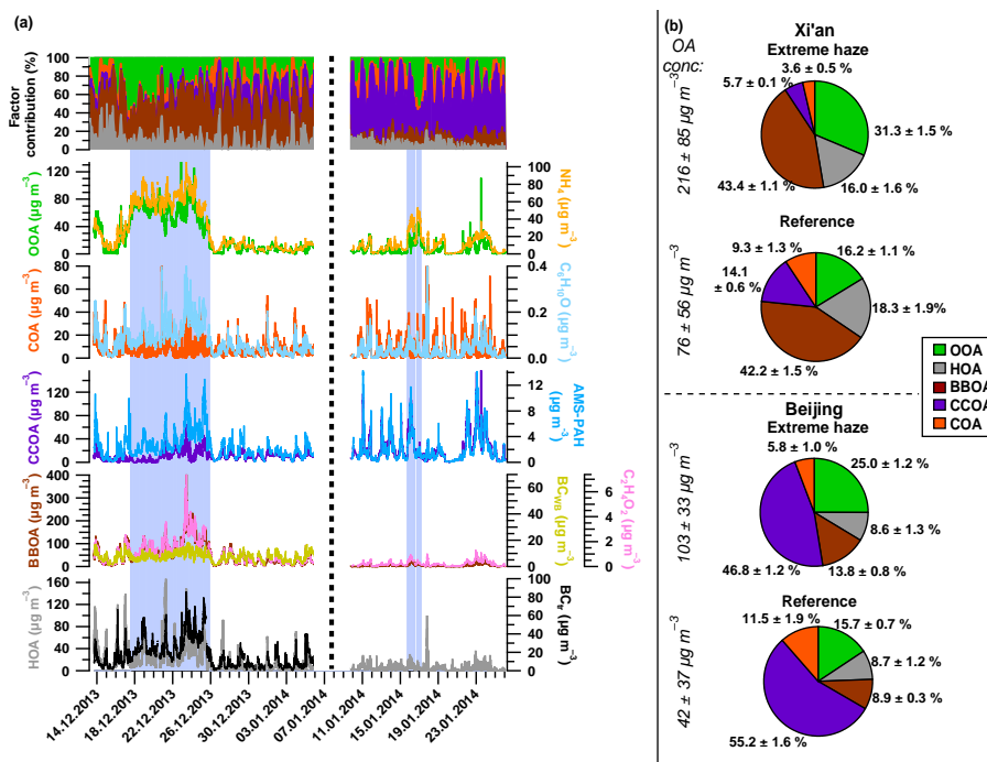
Figure 6. (a) Time series of the OA sources and the external tracers and relative contribution of the different sources over time; (b) mean relative contributions of the OA sources for the four periods of interest. Errors represent the standard deviation among all good a value combinations.
