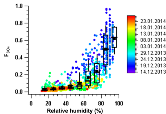
Figure 9. Sulfur oxidation ratio ( F_{\text{SO}_4} ) as a function of RH, colored by date. Mean (square), median (middle horizontal line), 25th and 75th percentiles (P25–P75, box) and 10th and 90th percentiles (P10–P90, whiskers) are reported for each RH bin (10% step).
