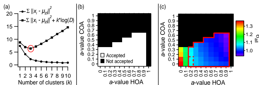
Figure 2. (a) The first term T1 (circles) and the total cost function CF ( T1 + T2 ) (squares) defined in Eq. (4) for increasing number of clusters ( k ); (b) final accepted a value range after applying the criteria 1 and 2; (c) color-coded quadratic sum of standard deviations between external tracers and correlated primary OA sources. The region surrounded with red line includes all final accepted a value combinations obtained from the study of the variability of the solution among 50 solutions with pseudo-randomly modified input matrix within twice its errors ( \mathbf{OA} \pm 2\mathbf{OA}_{\text{error}} ). The dashed line in the left lower corner shows the two a value combinations that would not have been considered as good solutions if smaller changes were allowed to the input matrix ( \mathbf{OA} \pm 1\mathbf{OA}_{\text{error}} ) and only 10 solutions were considered for the variability study.
