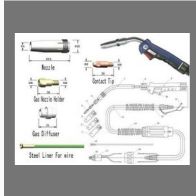
Mig Torch Accessories
