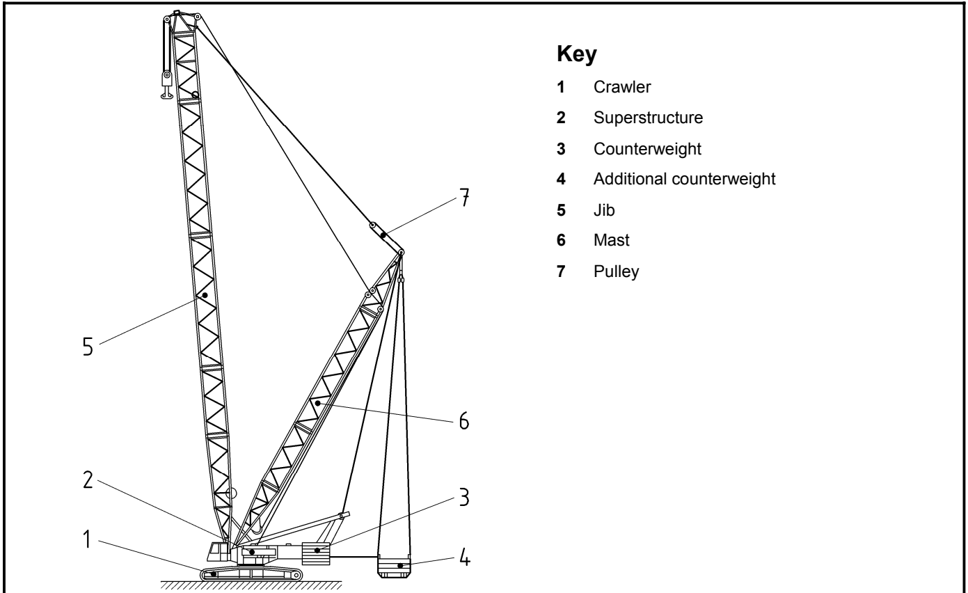
Figure B.2.1 — Examples of major parts
