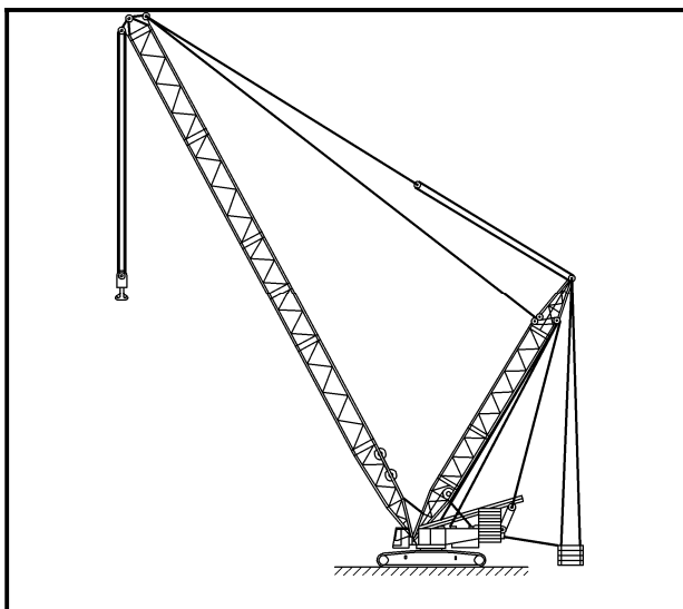
Figure A.7 — Crawler crane with additional counterweight
