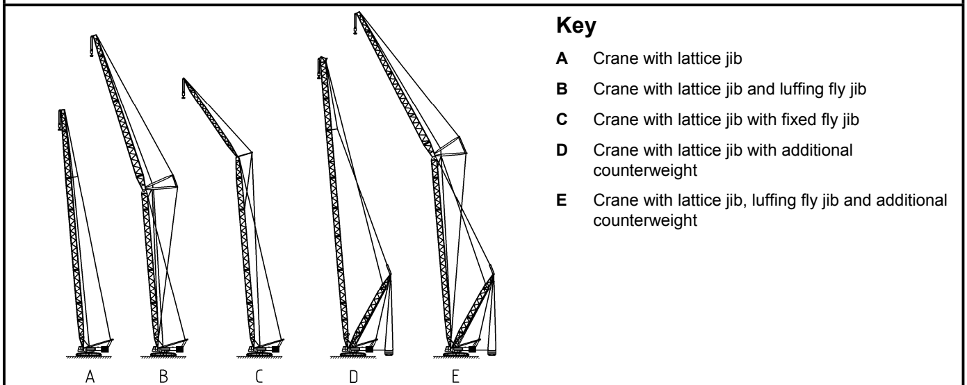
Figure B.2.2 — Examples of jibs and jib combinations
