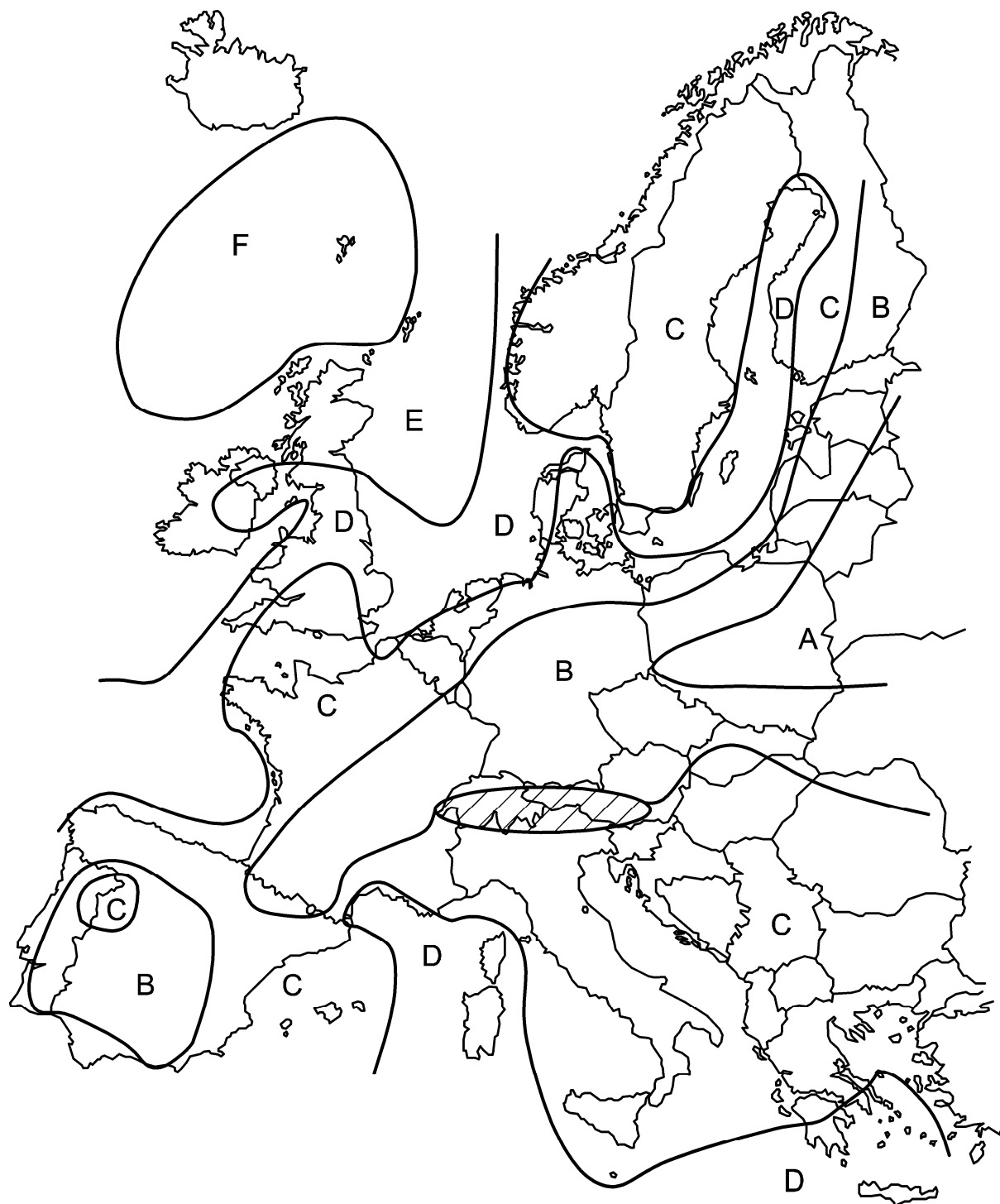
Figure N.3.1 — Regions where same mean storm wind velocities are applicable
