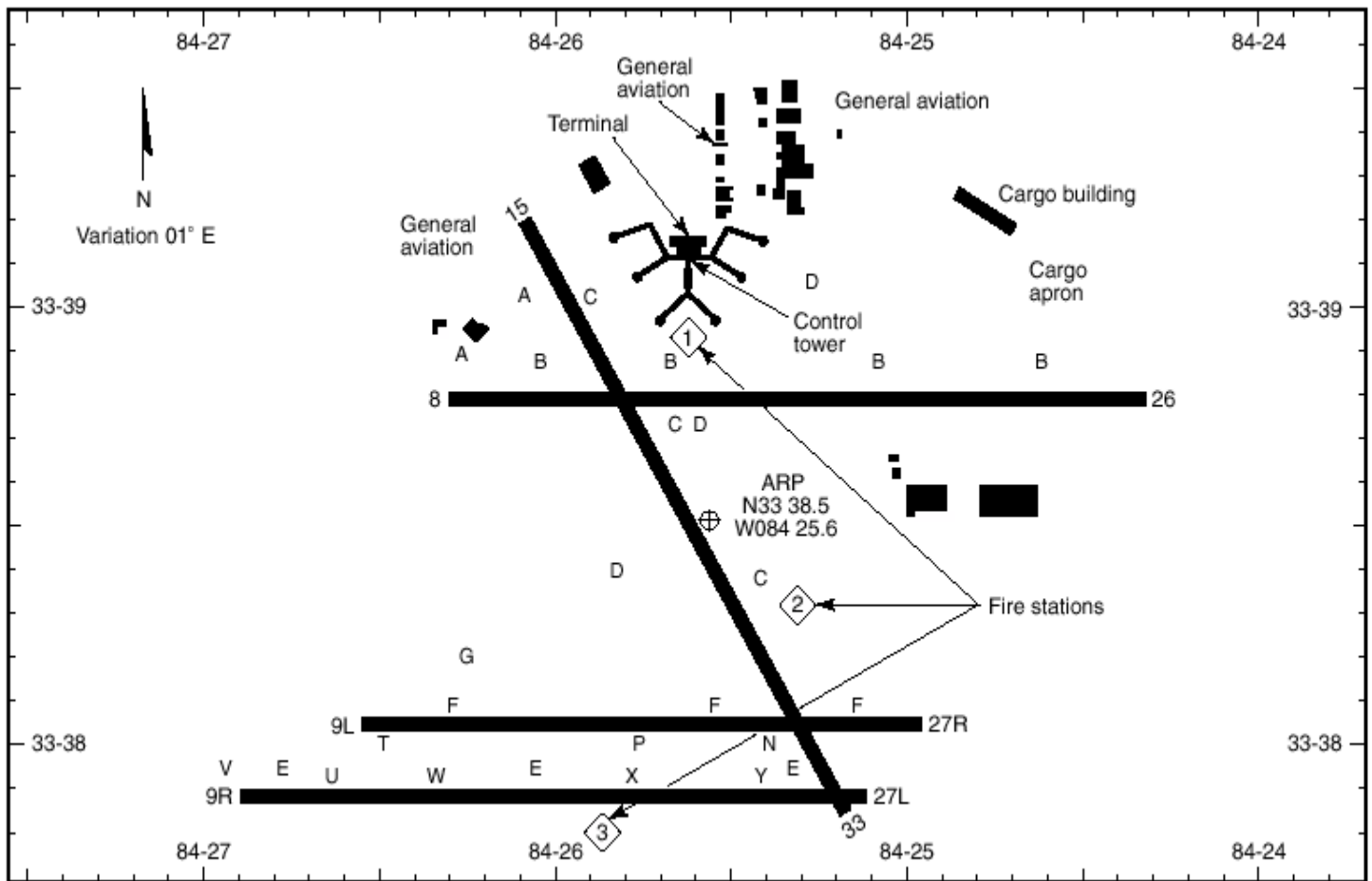
FIGURE 6.2.3 Example of Airport Fire Station Locations.
