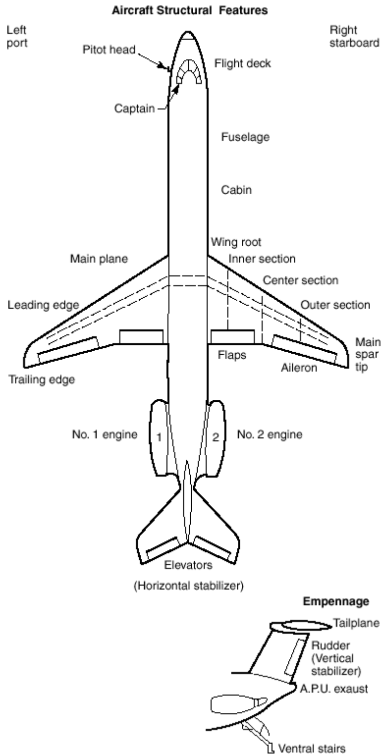
FIGURE 8.1.1 Nomenclature for Aircraft Structural Features.
