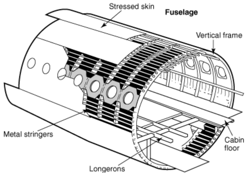
FIGURE 8.1.2 Fuselage Components.
