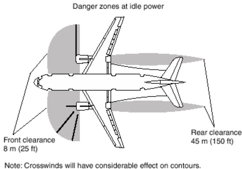
FIGURE 7.5.6 Engine Run Danger Areas.
