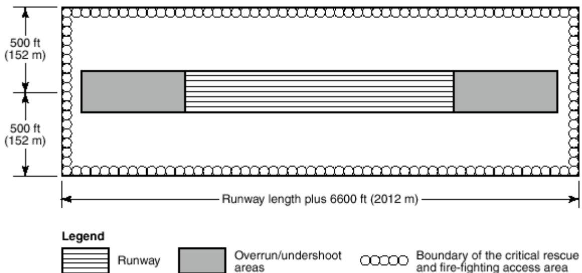
FIGURE 6.1.2 Critical Rescue and Fire-Fighting Access Area.
