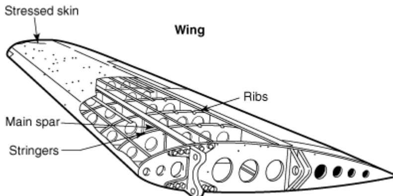
FIGURE 8.1.3 Wing Components.
