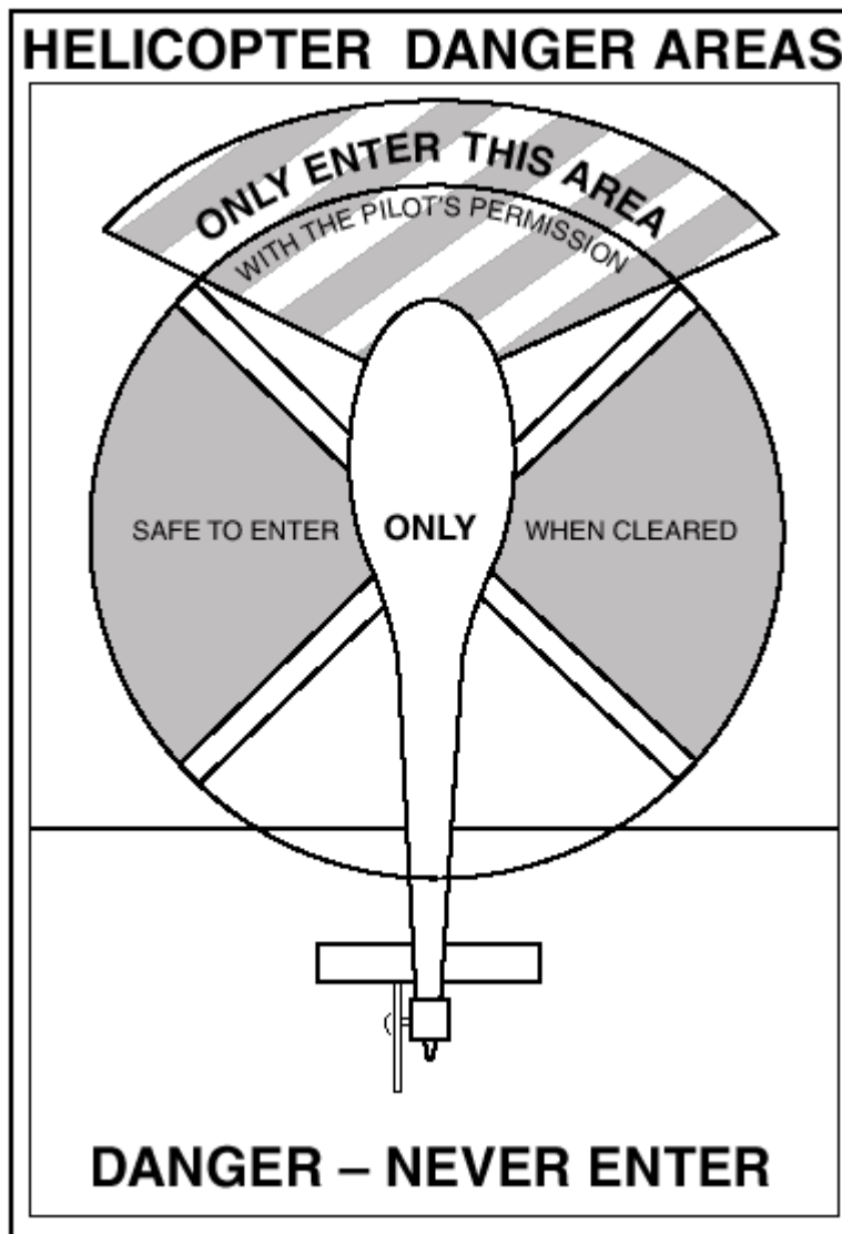
FIGURE 7.5.10(b) Helicopter Danger Areas.
