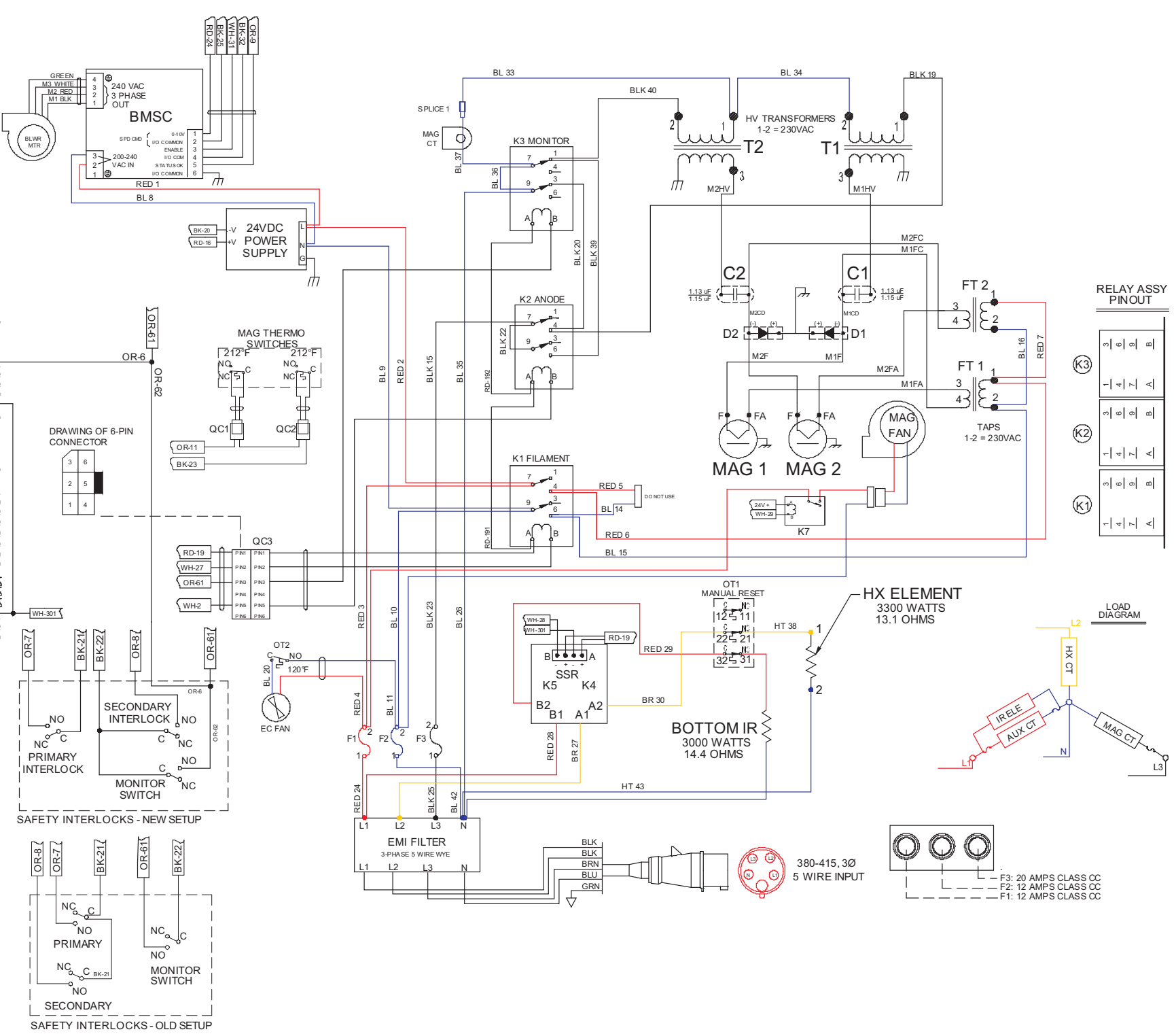
FIGURE 42: NGCEW (Tornado) Schematic
