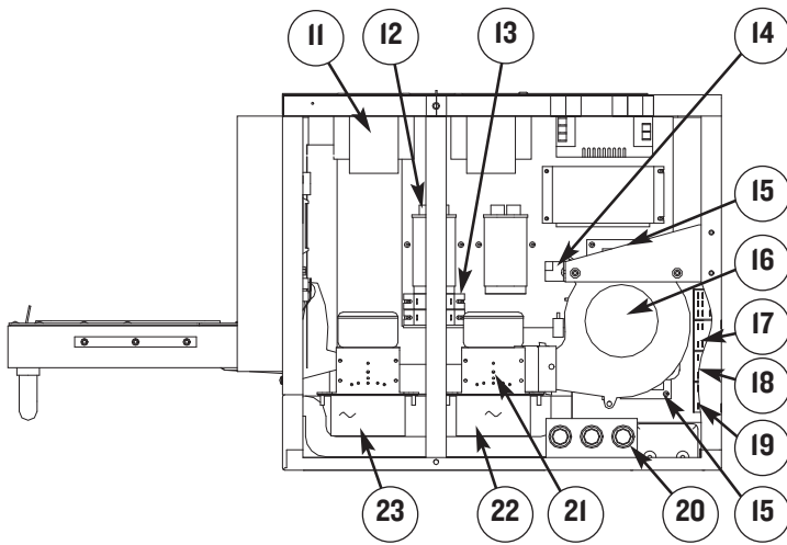
FIGURE 20: Microwave System Parts
