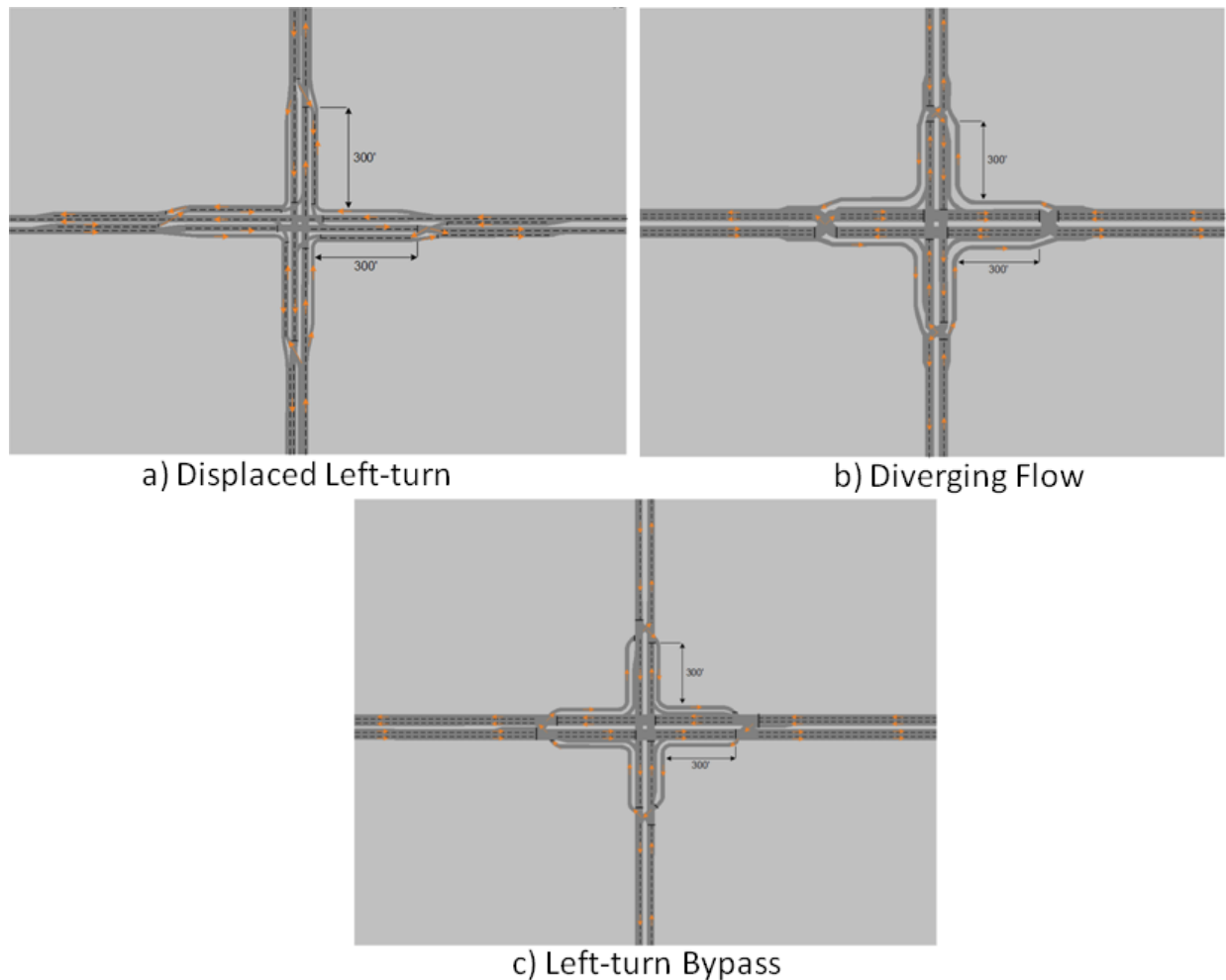
Figure 2- Unconventional Intersection Designs Description
