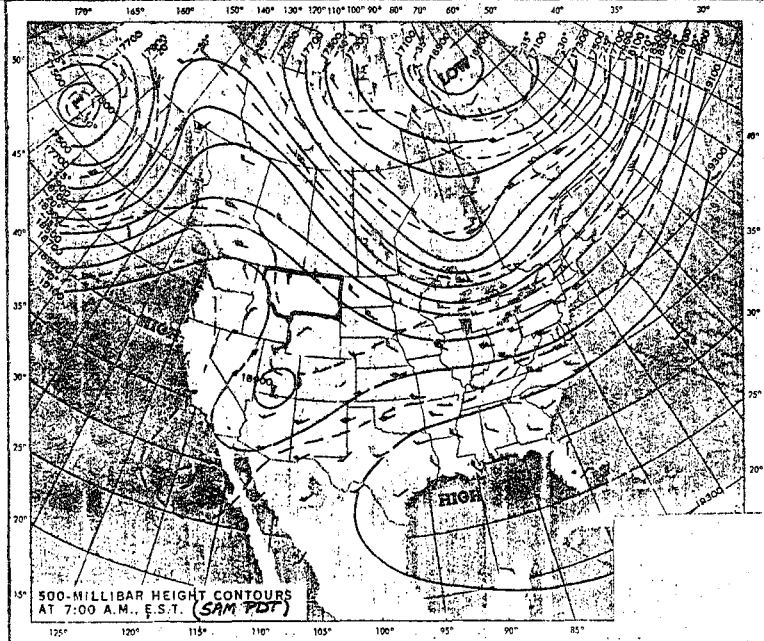
FIGURE 3. SURFACE AND 500-MB ANALYSES FOR 1200Z (5 AM PDT), SEPTEMBER 15, 1974 (EXTRACTED FROM DAILY WEATHER MAPS).
