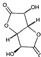
D-Glucaro-1,4:6,3-dilactone
