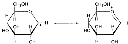
D-Glucopyranosylium
