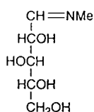
1-Deoxy-1-(methylimino)-D-xylitol
