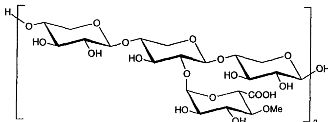
(4-O-Methyl-α-D-glucurono)-D-xylan
