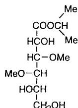
Isopropyl 3,4-di-O-methyl-L-mannonate
