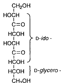
D-glycero-D-ido-Nono-3,6-diulose
