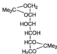
1,2:5,6- O -isopropylidene-D-mannitol
