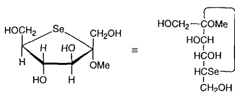
Methyl 5-seleno-α-D-fructofuranoside
