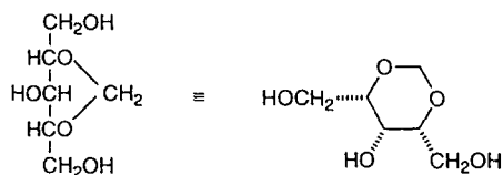
2,4- O -Methylenexylitol
