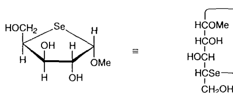
Methyl 4-seleno-α-D-xylofuranoside
