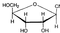
2,5-Anhydro-D-allonitrile
