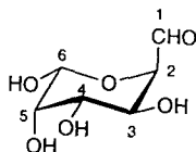
(6 R )-D-gluco-Hexodialdo-6,2-pyranose
