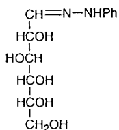
D-Glucose phenylhydrazone
