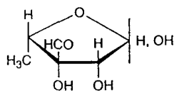
Streptose
