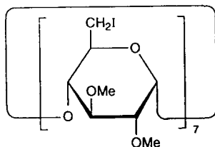
Heptakis(6-deoxy-6-iodo-2,3-di-O-methyl)cyclomaltoheptaose
