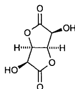
L-Mannaro-1,4:6,3-dilactone
