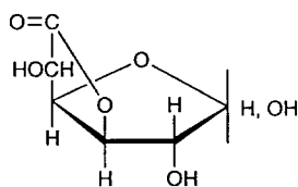
D-Glucufuranurono-6,3-lactone
