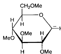
1,5-Anhydro-2,3,4,6-tetra-O-methyl-D-glucitol-1-ide
